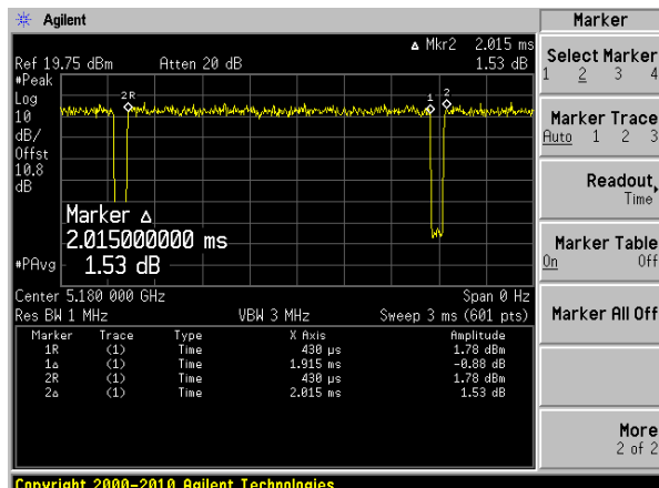
802.11n20 mode
