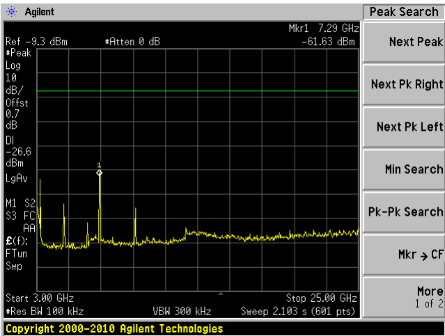
Middle channel 3-25 GHz
