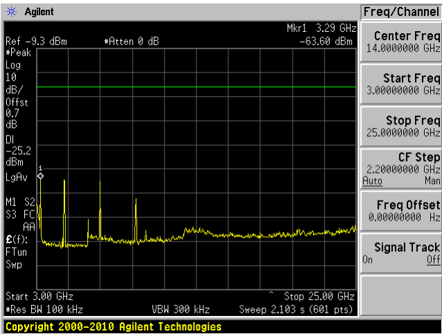
High channel 3-25 GHz
