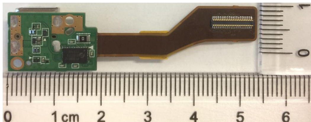
RFPC, USB-Back
