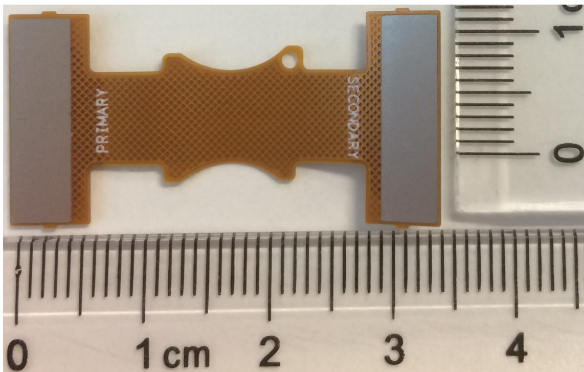
FPC, INTER-PROCESSOR-Back
