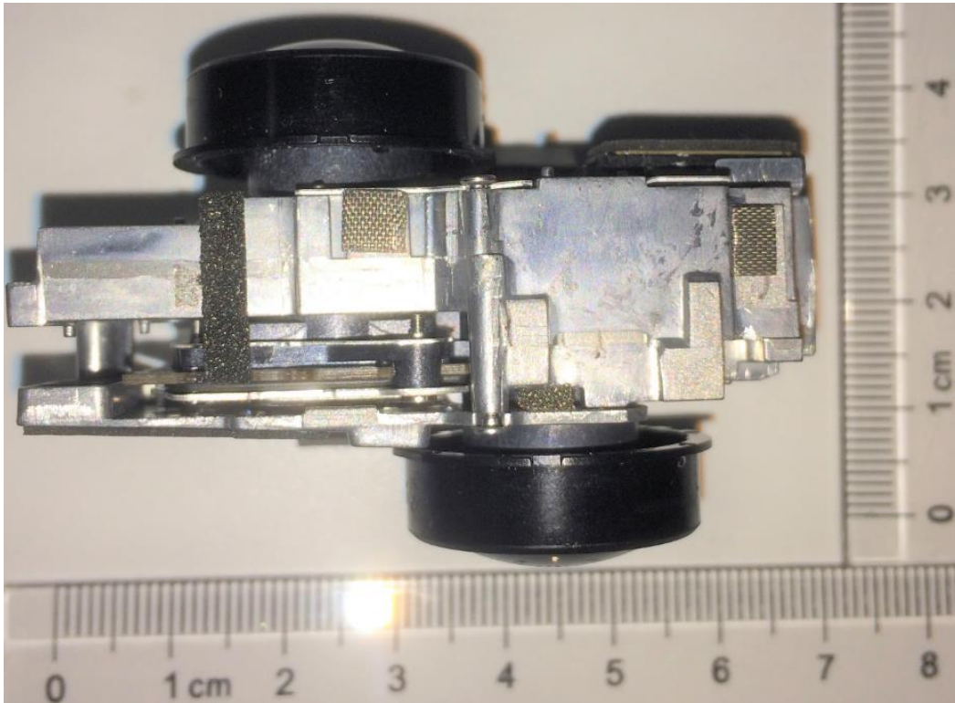
Lens Module-Back
