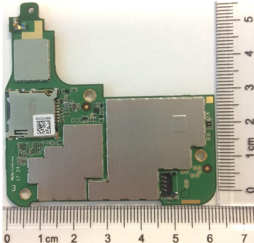
PCBA, MAIN, PRIMARY- Back with shield removed
