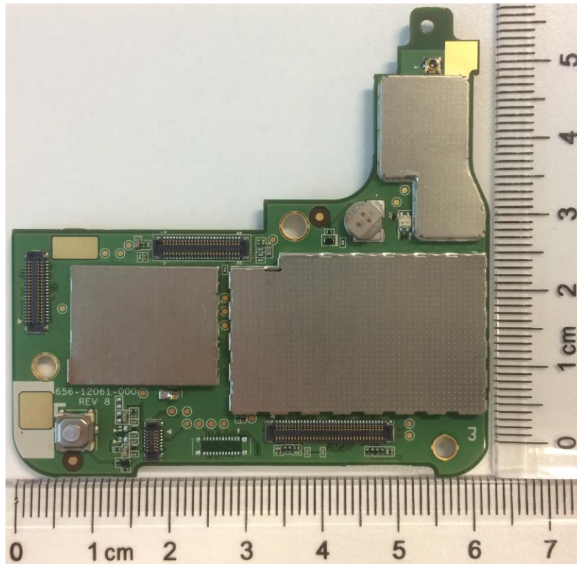
PCBA, MAIN, PRIMARY- Front with shield removed
