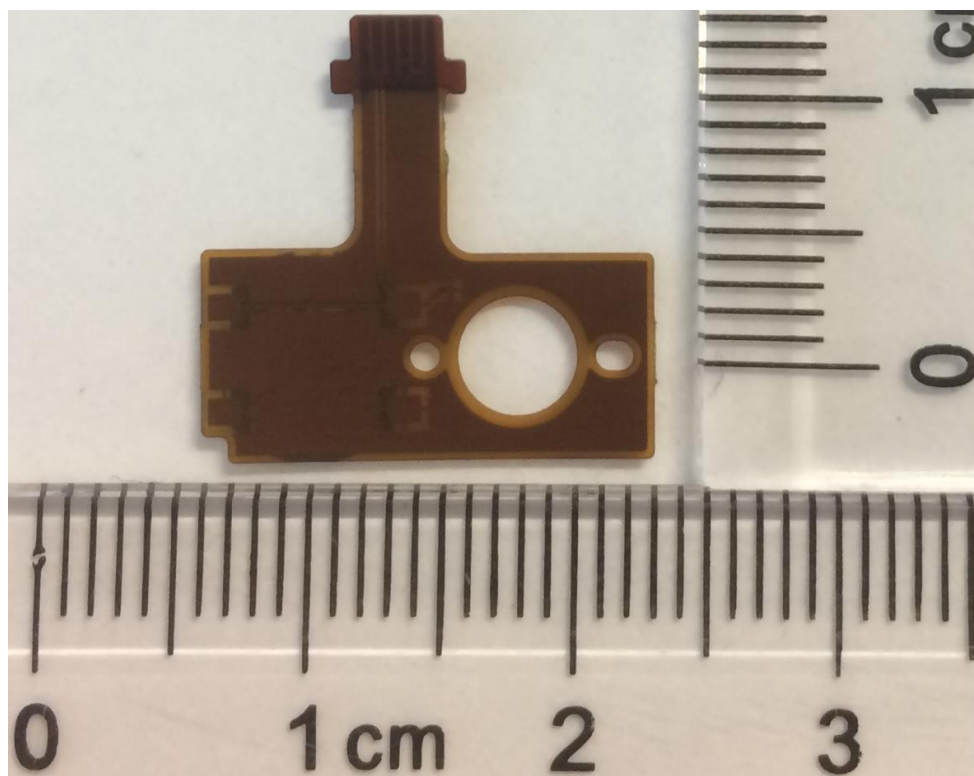
FPC, BUTTONS-Back
