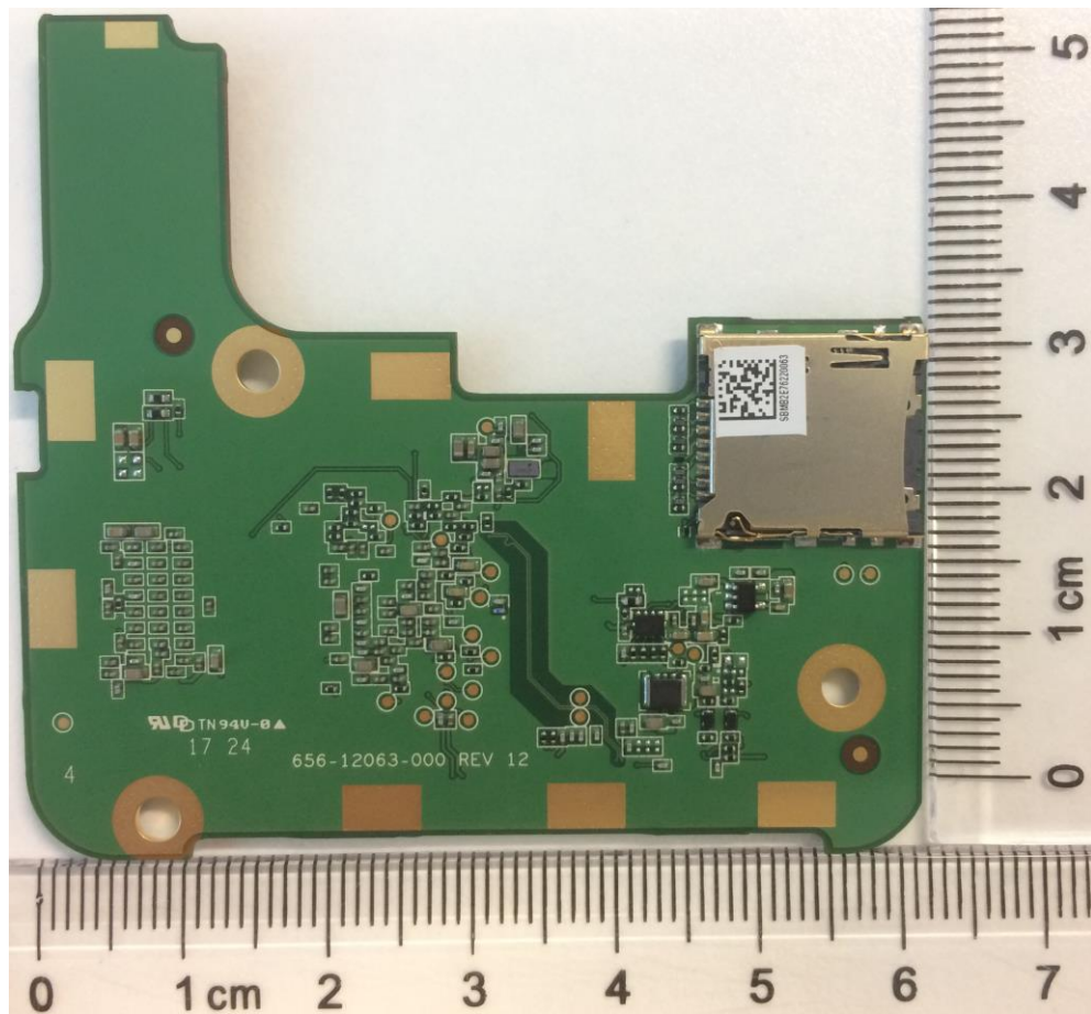
PCBA, MAIN, SECONDARY-Back
