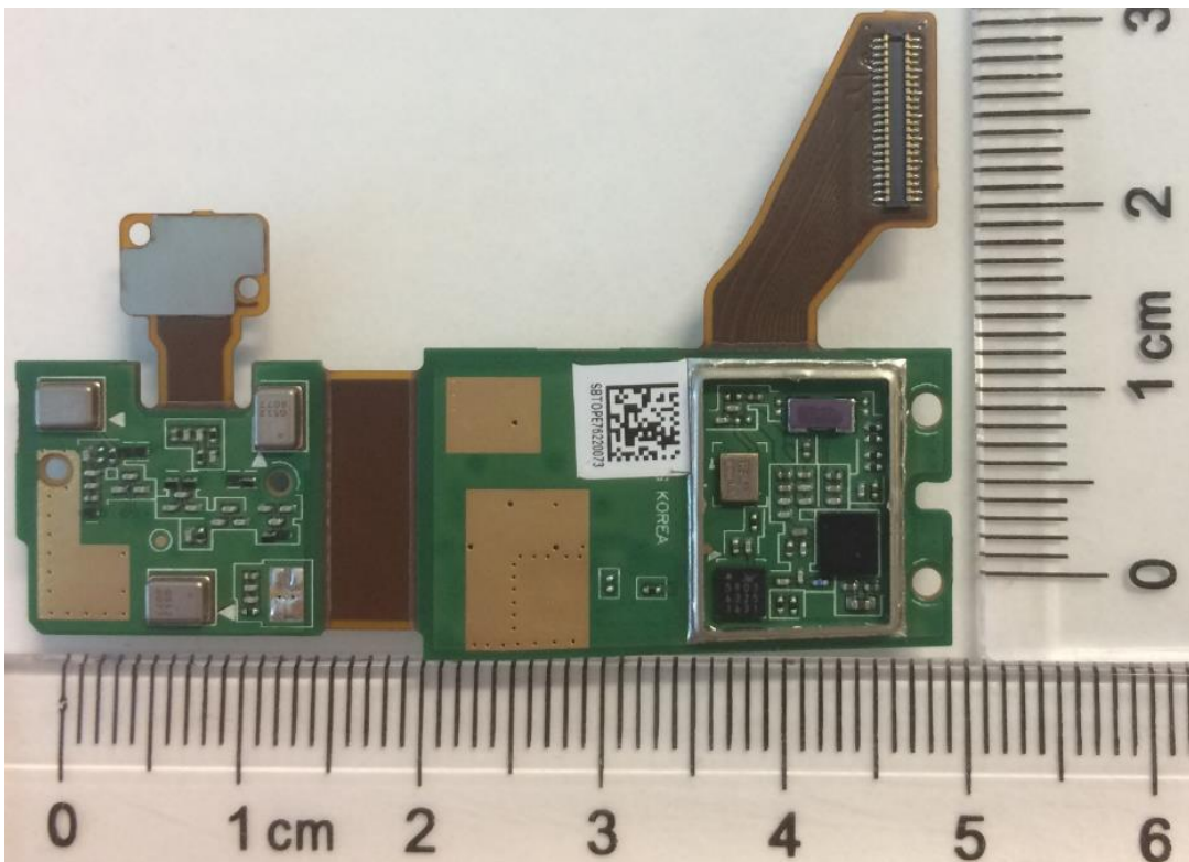
RFPC, TOP-Back with shield removed
