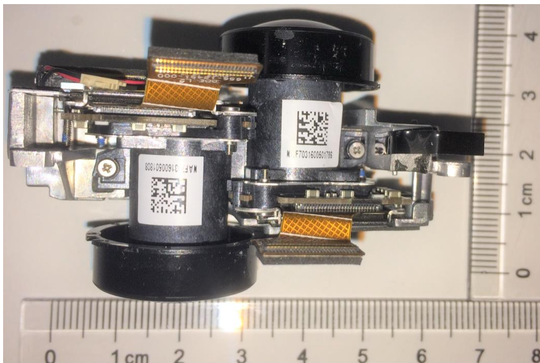
Lens Module-Back
