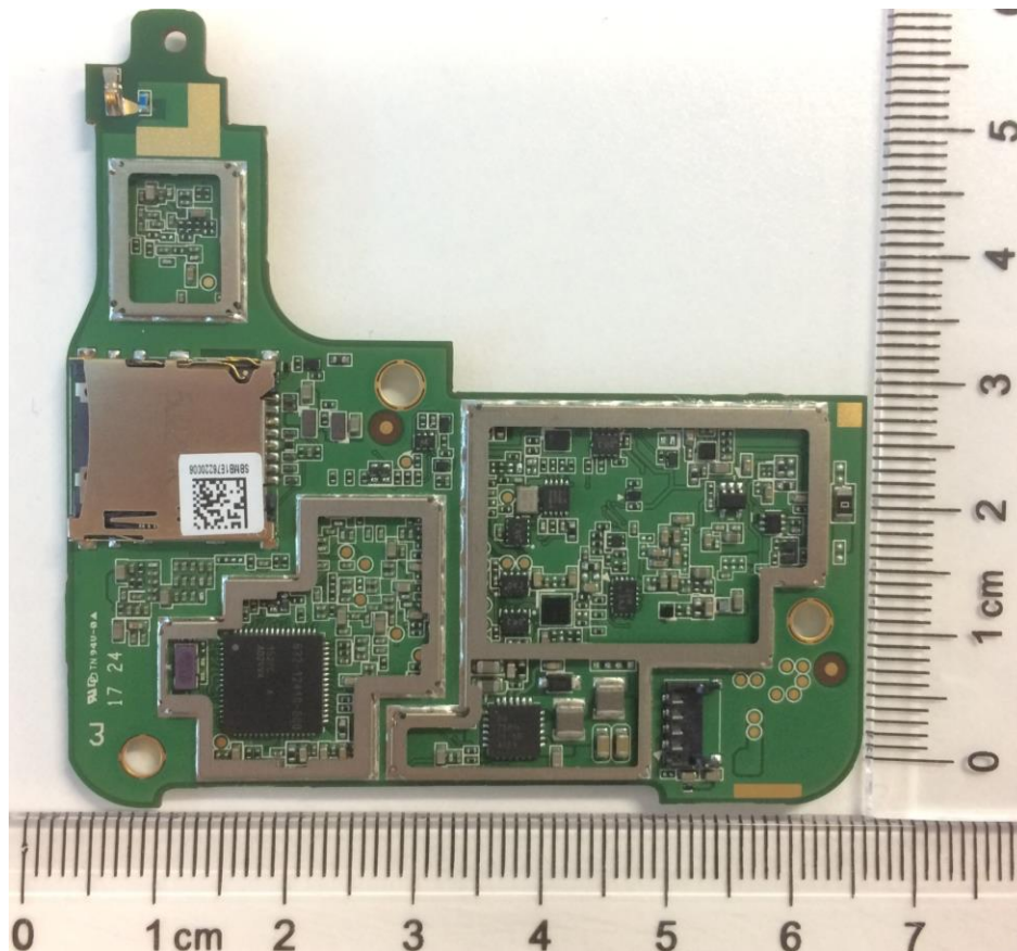
PCBA, MAIN, PRIMARY- Back with shield removed
