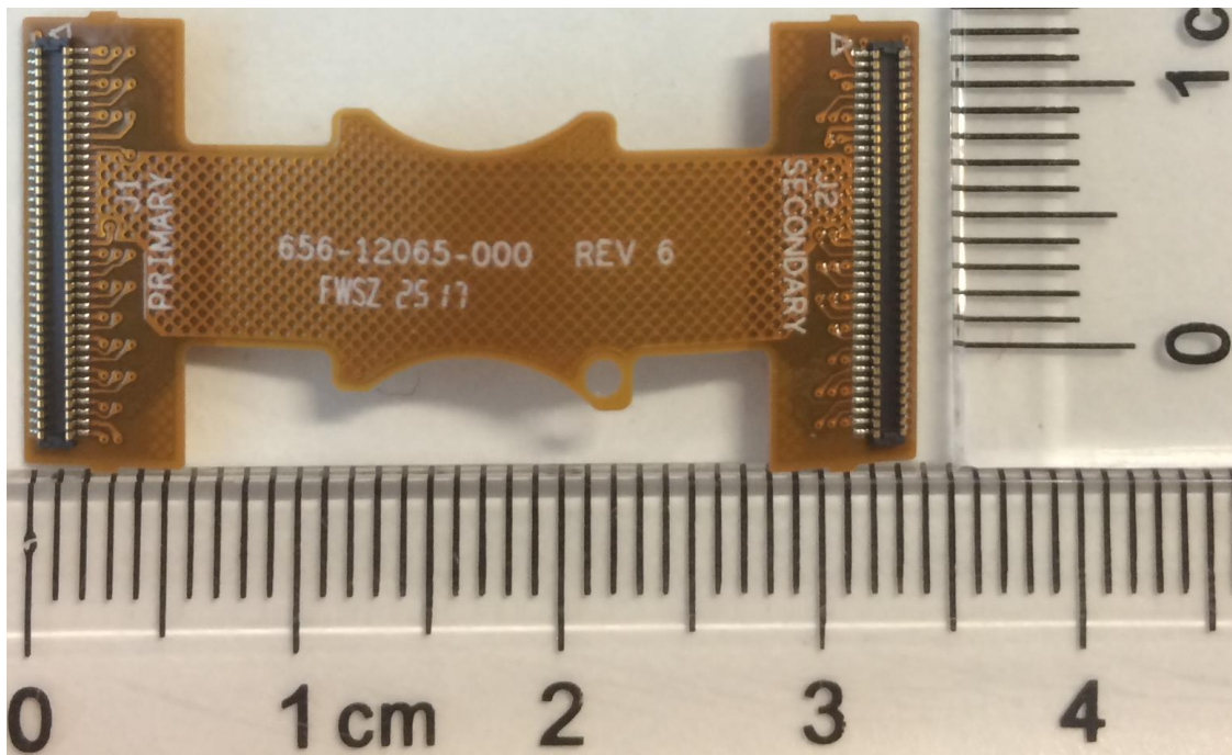
FPC, INTER-PROCESSOR-Back
