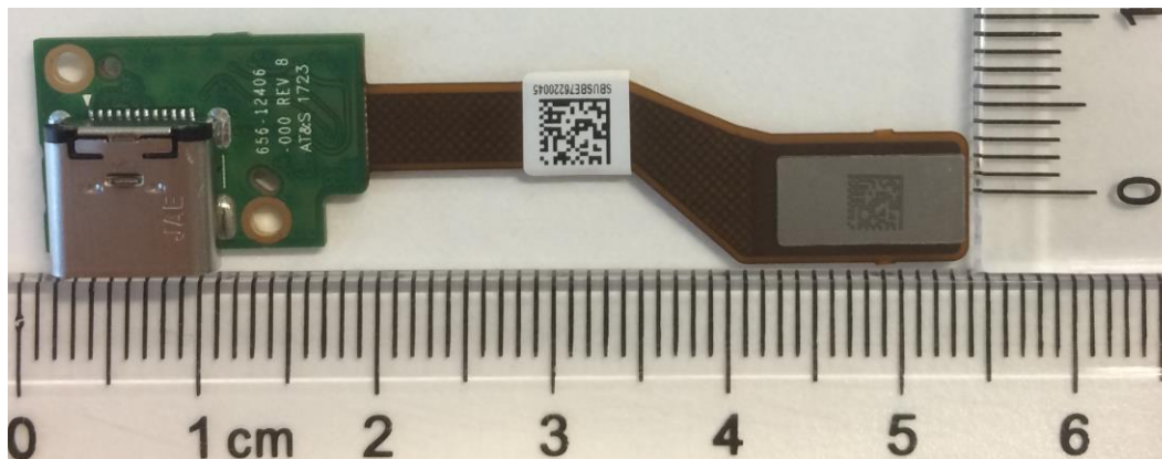
RFPC, USB-Back
