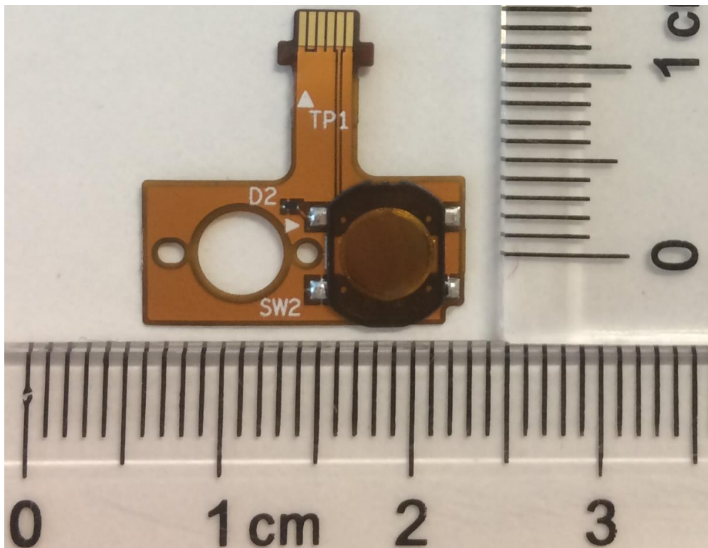
FPC, BUTTONS-Back
