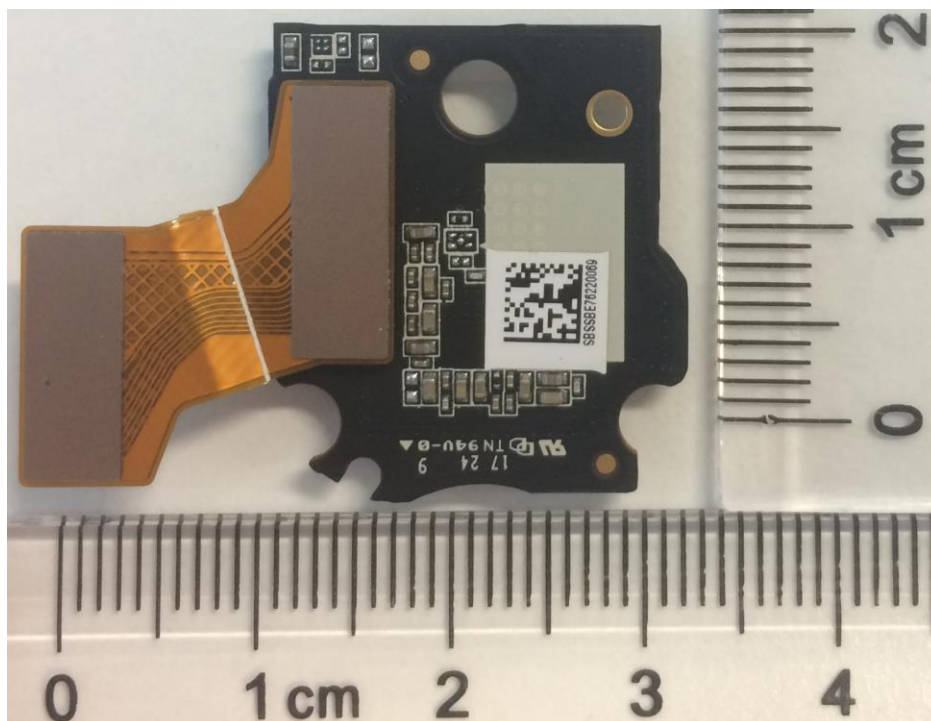
PCBA, IMAGE SENSOR and FPC, JUMPER, IMAGE SENSOR- Back
