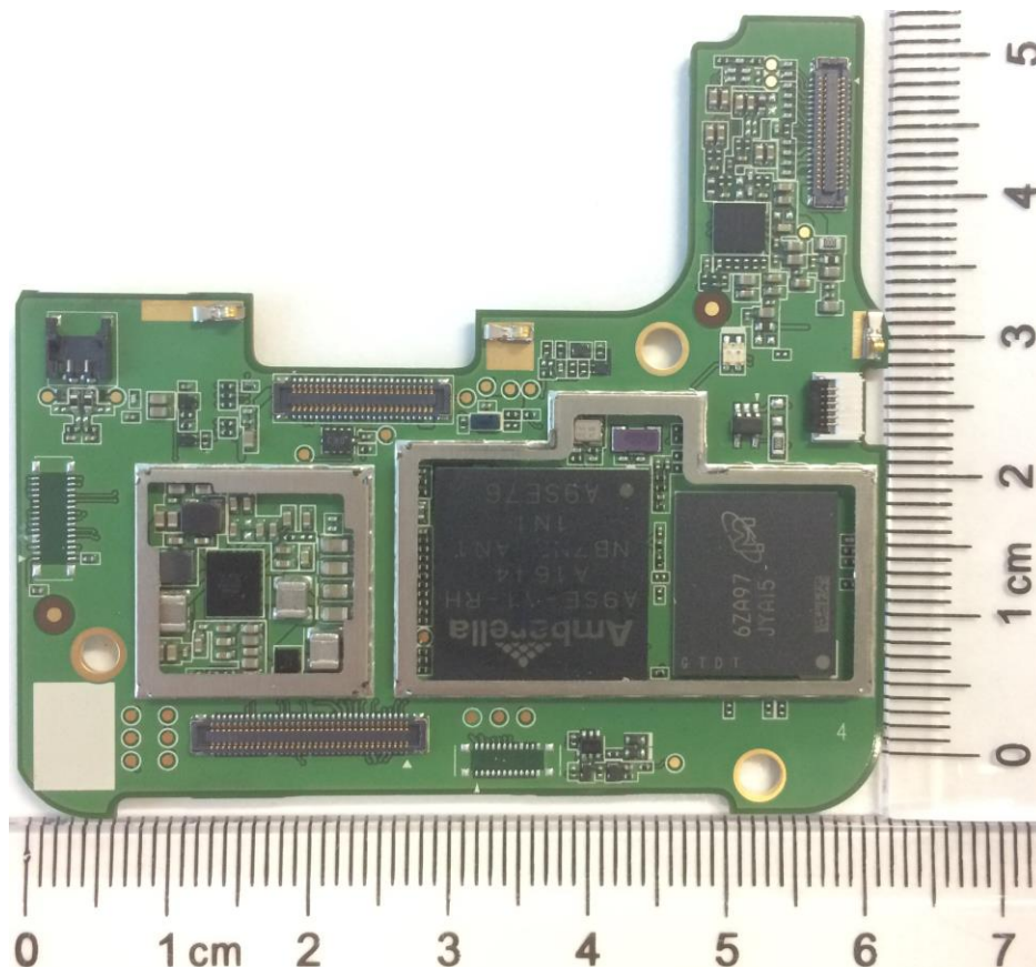
PCBA, MAIN, SECONDARY-Front with shield removed
