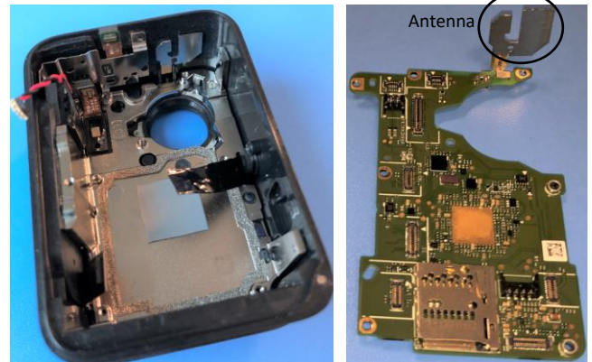
BT/WIFI antenna location, SPBL1
