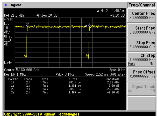
802.11n20 mode
