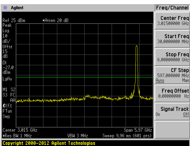
5290 MHz (30MHz-6GHz)
