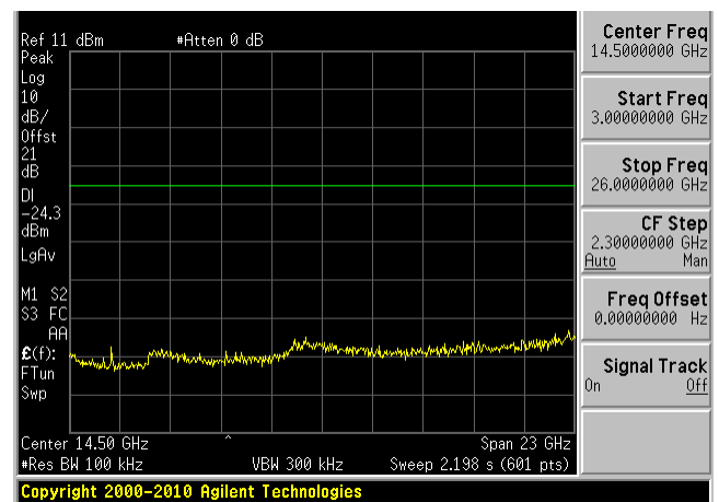
High Channel 3 GHz – 26 GHz
