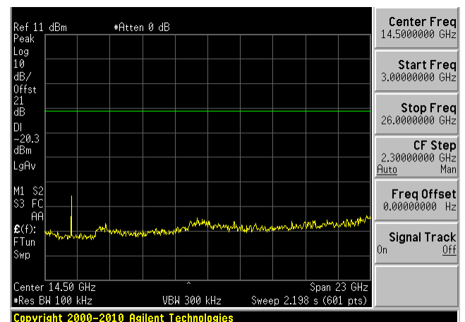
Middle Channel 3 GHz – 26 GHz
