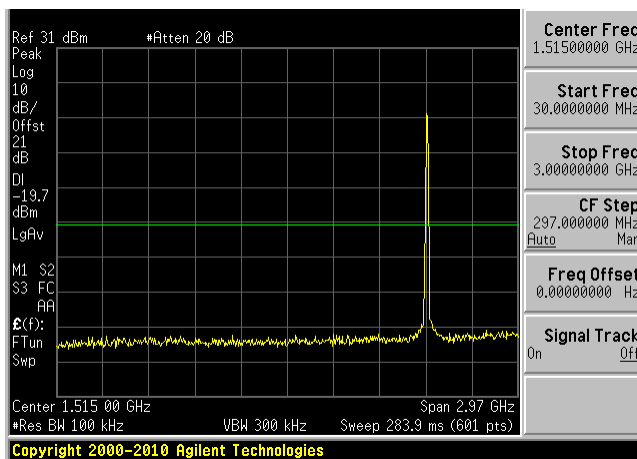
Low Channel 30MHz – 3 GHz
