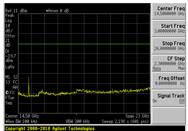
Low Channel 3 GHz – 26 GHz
