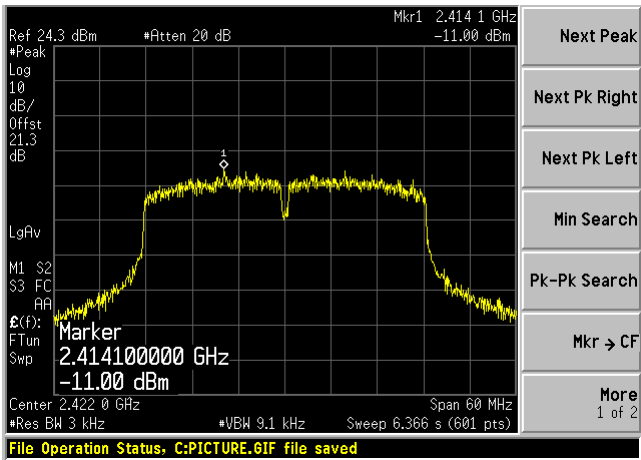
Low Channel 2422 MHz
