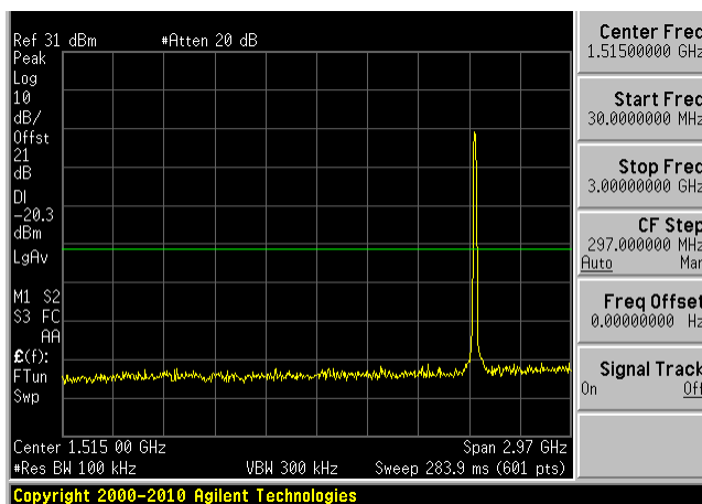
Middle Channel 30 MHz – 3 GHz
