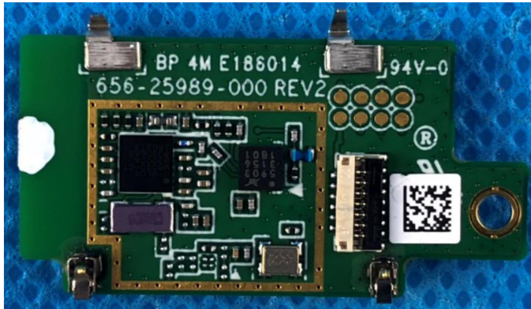
656-25989-000 PCB, GPS- SPTM1(Version S) -Back
