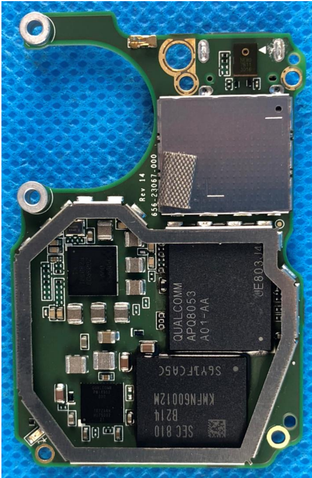
656-23067-000 PCBA, MAIN- SPTM1(version W)- Front with shield
