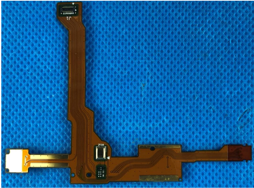
656-26058-000 FPC, MIC+BUTTON FLEX- SPTM1(Version S) -Back
