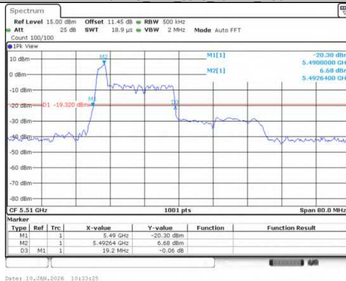
11AX40SISO Ant1 5510 52Tone RU37
