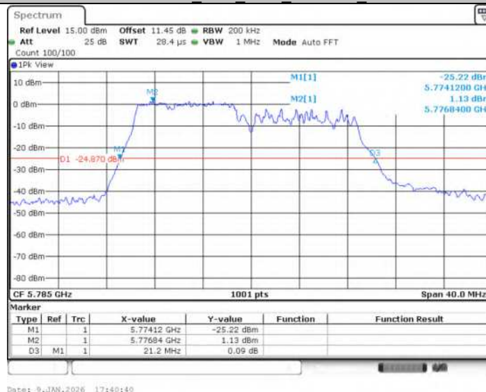
11AX20SISO Ant1 5785 242Tone RU61
