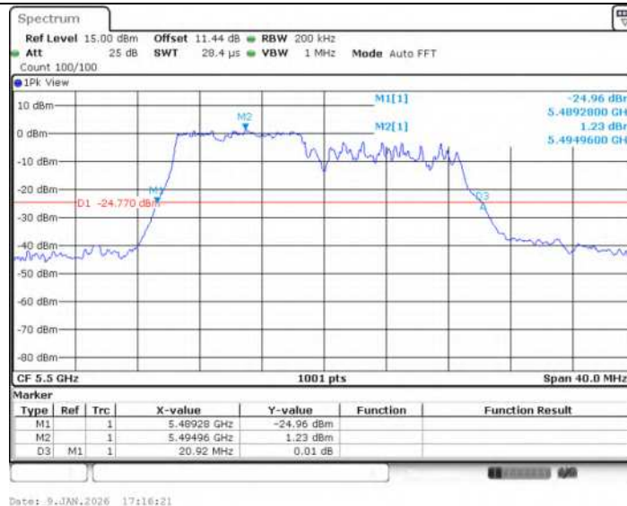
11AX20SISO Ant1 5500 242Tone RU61
