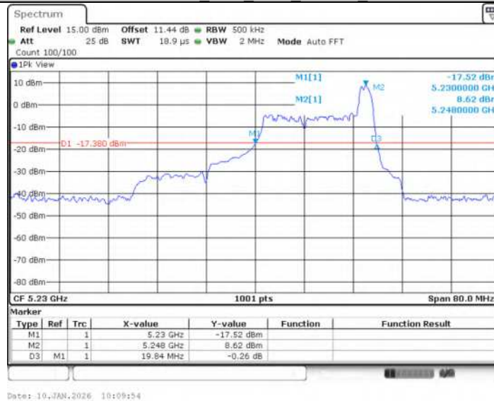
11AX40SISO Ant1 5230 52Tone RU44
