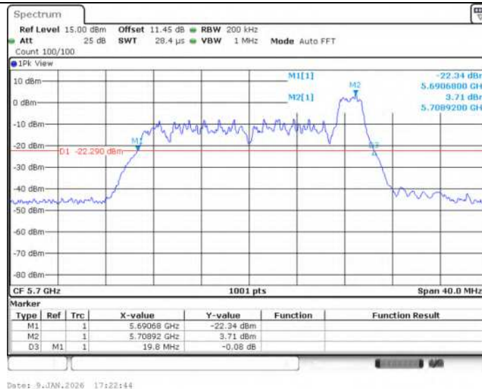
11AX20SISO Ant1 5700 52Tone RU40
