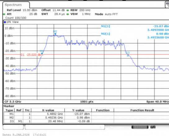
11AX20SISO Ant1 5500 106Tone RU53
