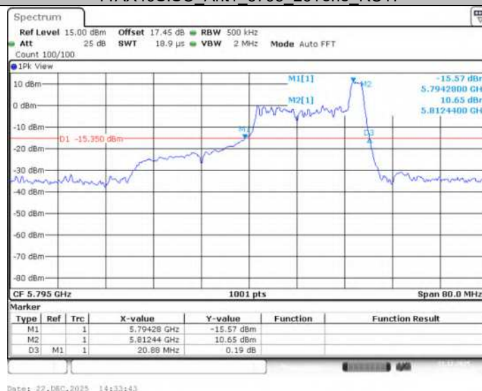
11AX40SISO Ant1 5795 52Tone RU44
