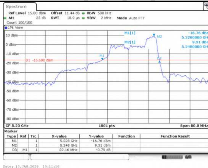
11AX40SISO Ant1 5230 106Tone RU56
