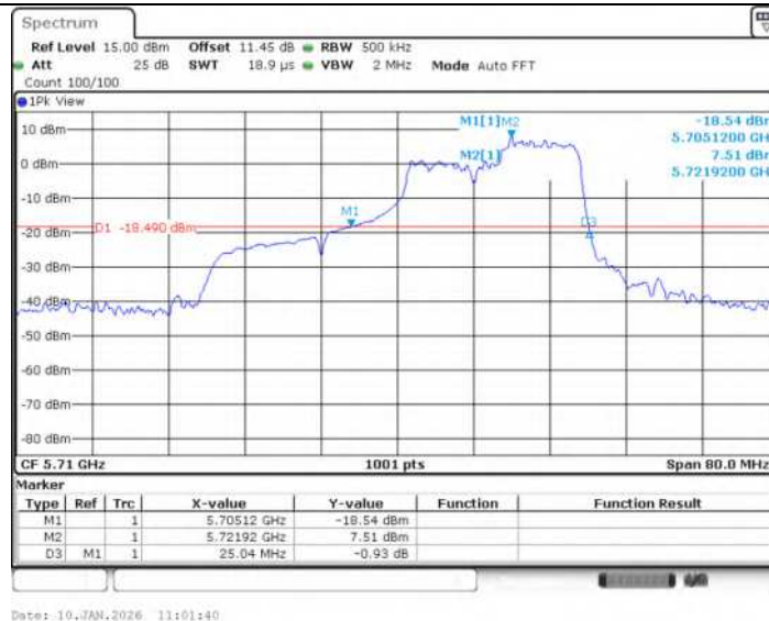
11AX40SISO Ant1 5710 242Tone RU62
