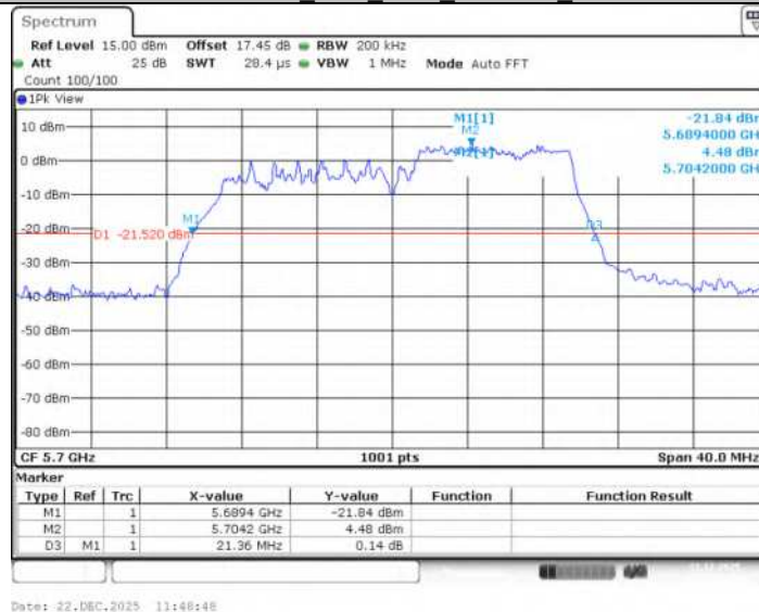
11AX20SISO Ant1 5700 242Tone RU61
