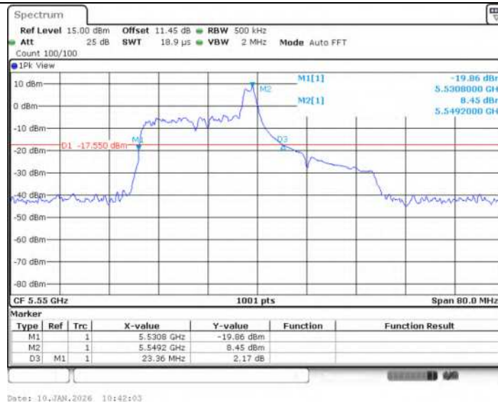
11AX40SISO Ant1 5550 52Tone RU40
