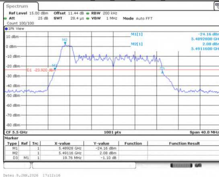
11AX20SISO Ant1 5500 52Tone RU37
