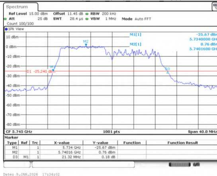
11AX20SISO Ant1 5745 242Tone RU61
