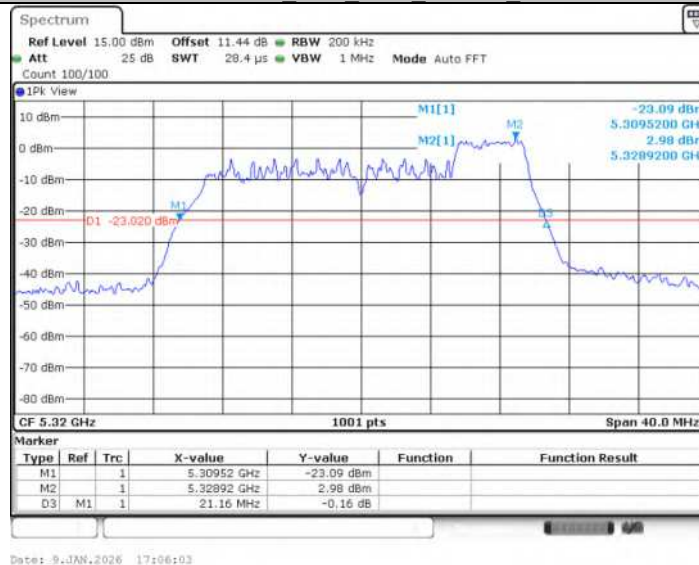
11AX20SISO Ant1 5320 106Tone RU54
