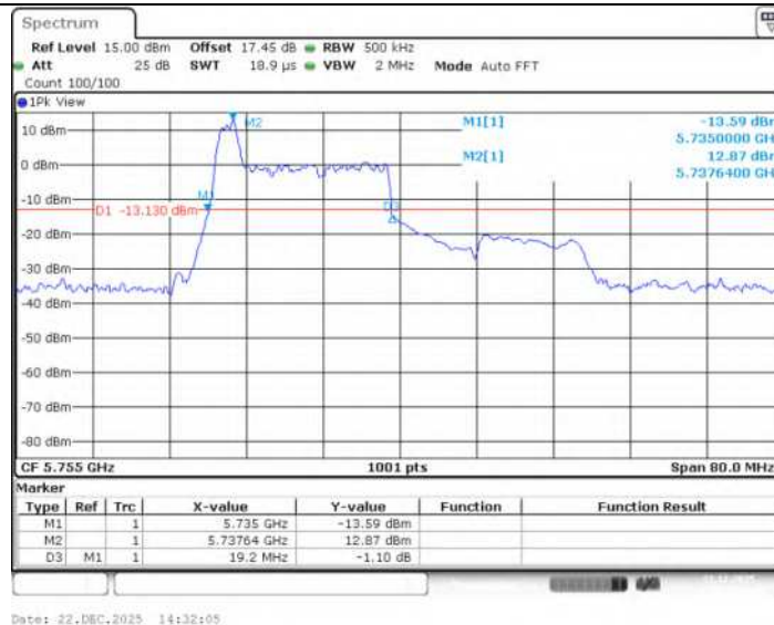
11AX40SISO Ant1 5755 52Tone RU37
