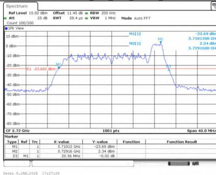
11AX20SISO Ant1 5720 52Tone RU40
