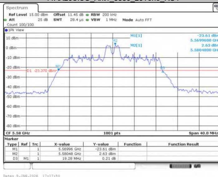
11AX20SISO Ant1 5580 52Tone RU38
