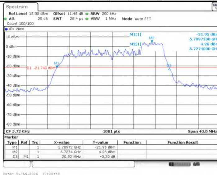
11AX20SISO Ant1 5720 106Tone RU54
