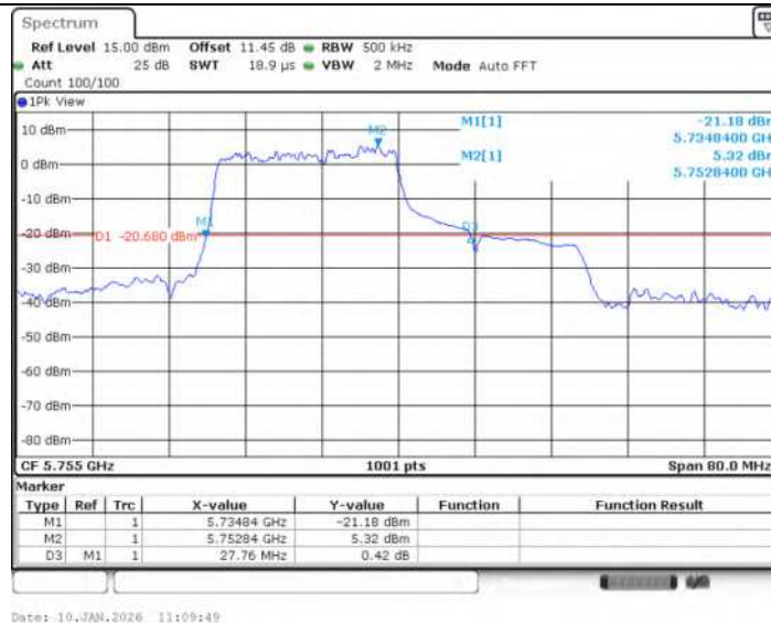
11AX40SISO Ant1 5755 484Tone RU65
