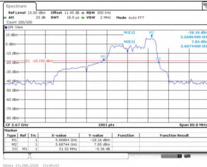
11AX40SISO Ant1 5670 106Tone RU56
