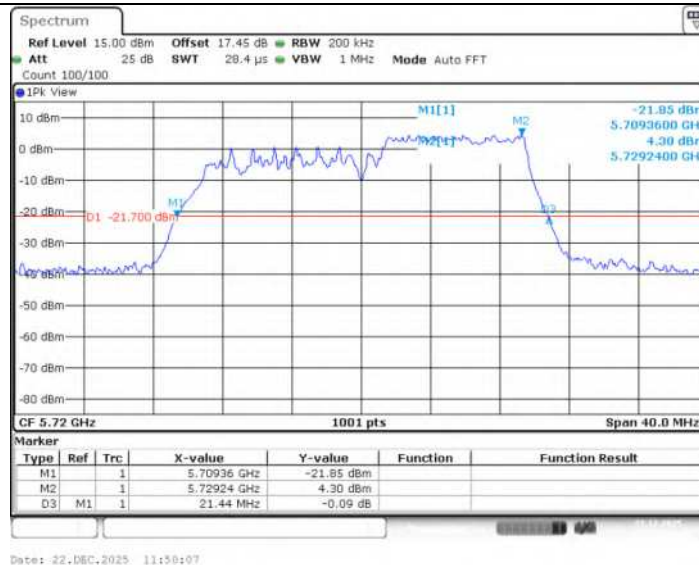
11AX20SISO Ant1 5720 242Tone RU61
