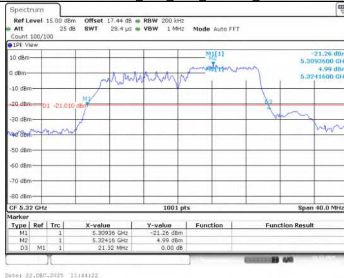
11AX20SISO Ant1 5320 242Tone RU61
