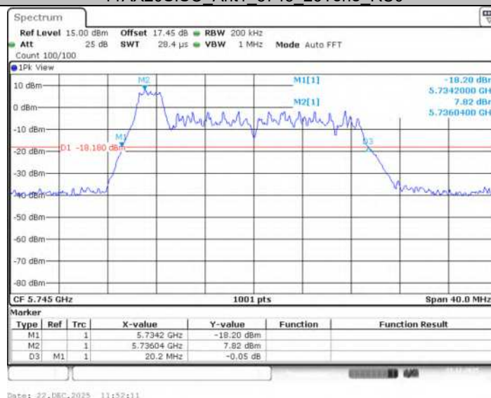
11AX20SISO Ant1 5745 52Tone RU37
