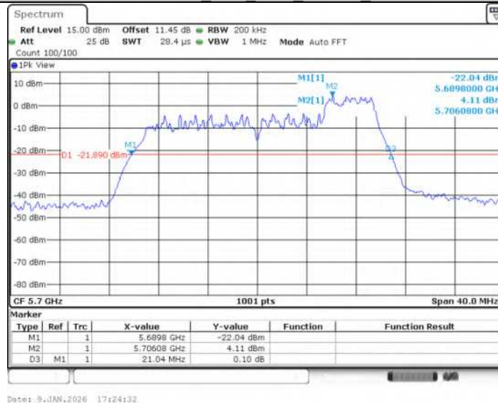
11AX20SISO Ant1 5700 106Tone RU54
