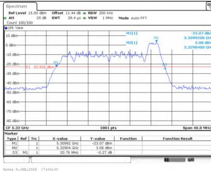
11AX20SISO Ant1 5320 52Tone RU40
