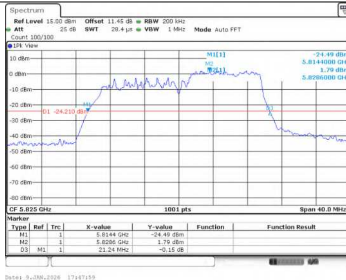
11AX20SISO Ant1 5825 242Tone RU61
