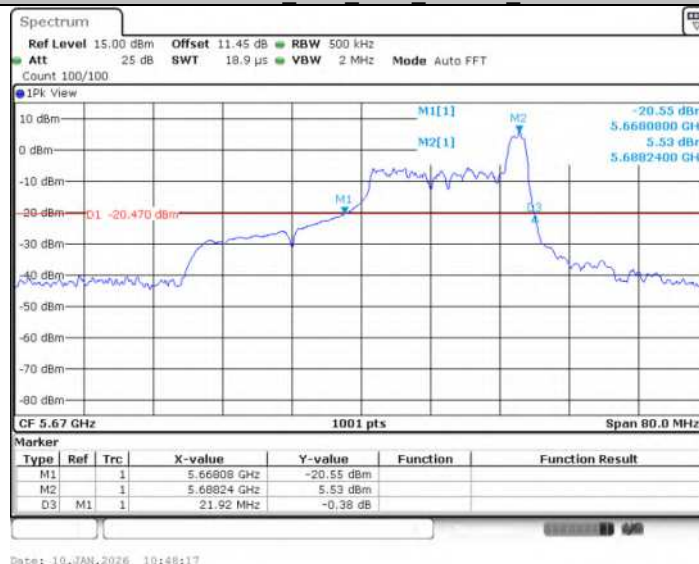
11AX40SISO Ant1 5670 52Tone RU44
