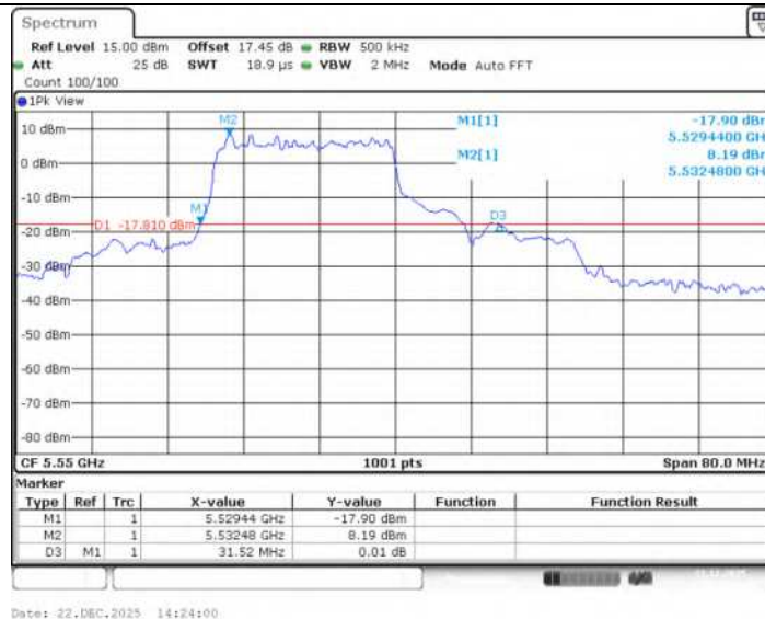
11AX40SISO Ant1 5550 484Tone RU65
