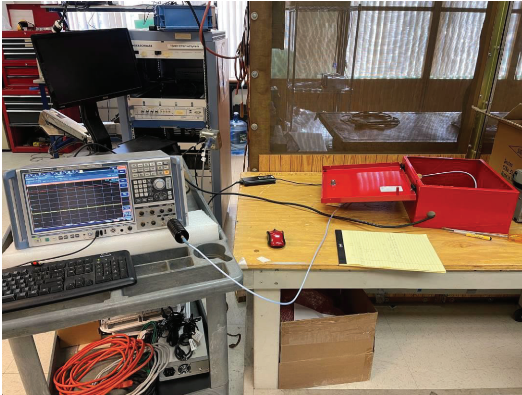
Test Setup Below 30 MHz
