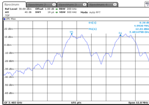
Figure 2. Plot of the Carrier Frequency Separation (Conducted)
