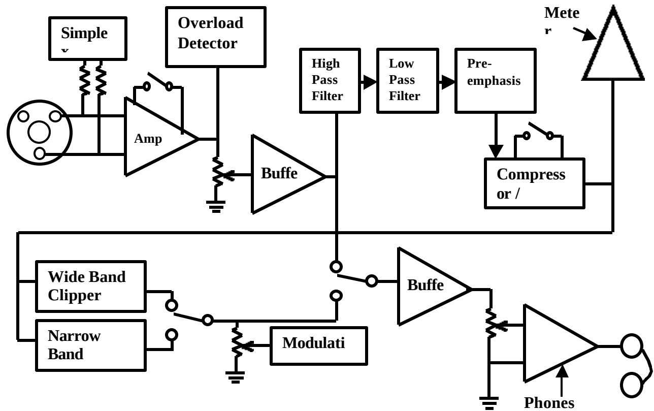
Figure 4. Audio Sub-system Block Diagram.
