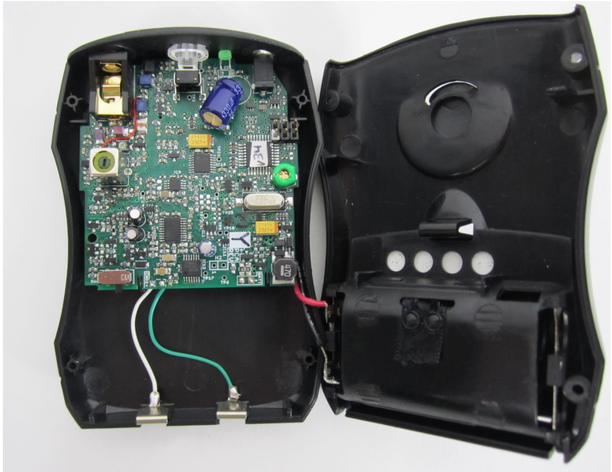
PC Board Component Side
