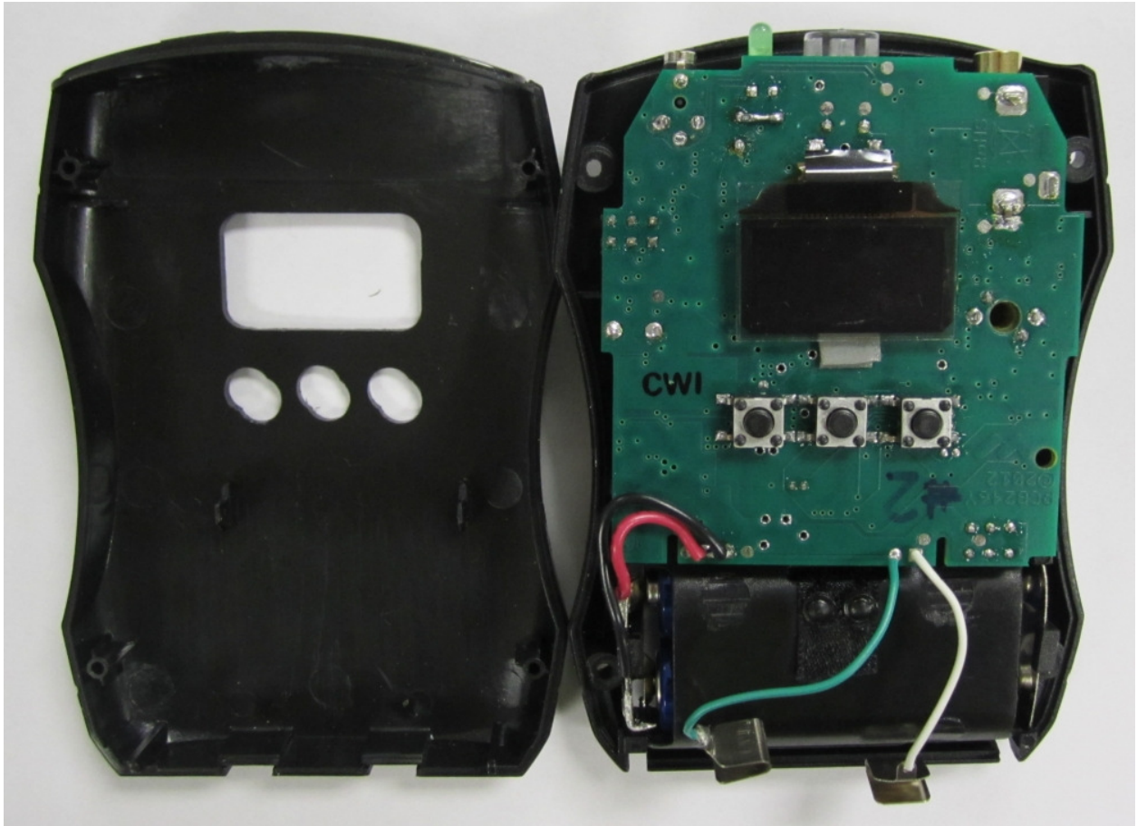
PC Board Solder side
