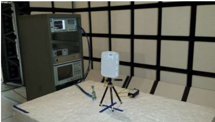
40000 TO 50000 MHz RADIATED EMISSIONS
