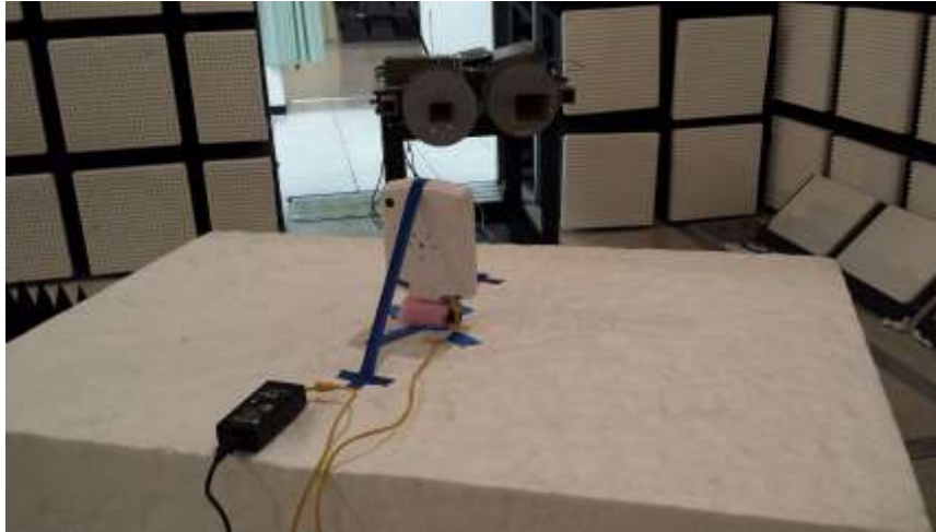
26000 TO 40000 MHz RADIATED EMISSIONS
