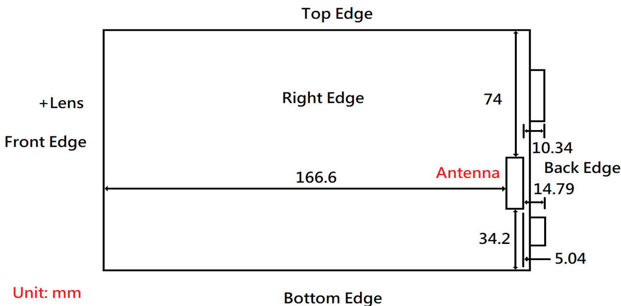
Photograph 15. Antenna position of EUT
