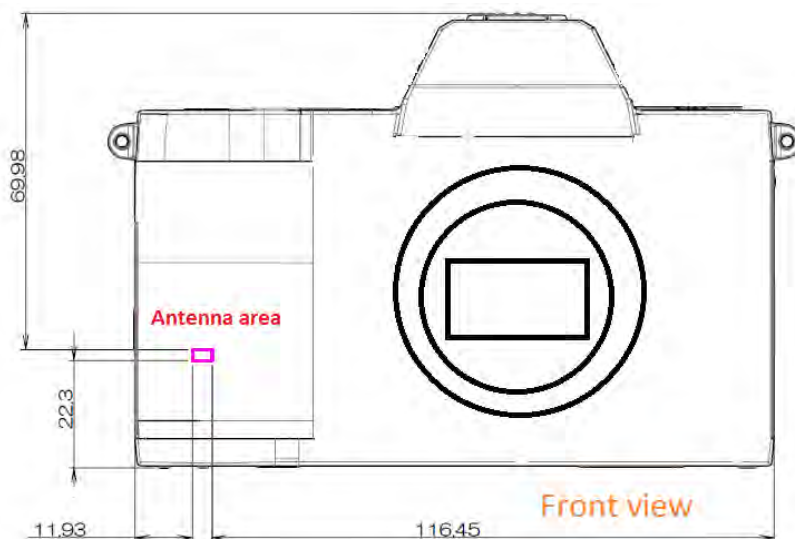
Fig.11 Antenna location
