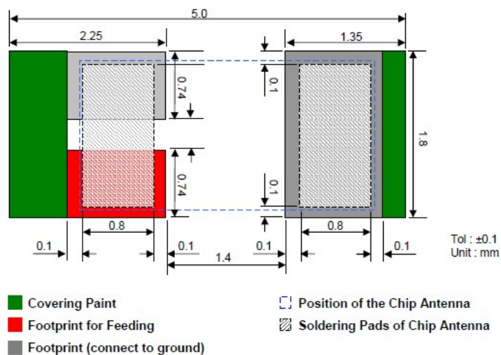
Fig. 4 Soldering Pads Dimension and Footprint
