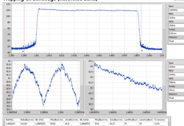
BT-BR(1Mbps) 2441MHz Hopping Ch Bandedge (Restricted Band)
