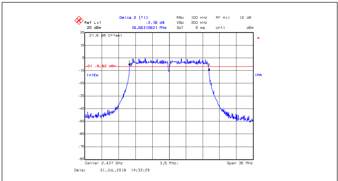
Plot 5.2.4.8. 6 dB Bandwidth, 16-QAM Modulation, 24 Mbps, Channel 6, 2437 MHz
