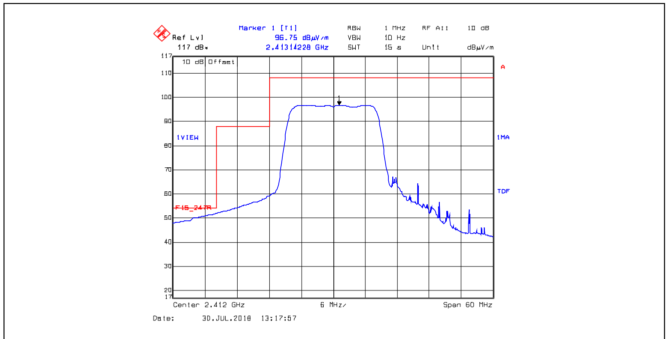
Plot 5.4.4.3.2. Band-Edge Radiated Emissions, EUT with 2.7 dBi Surface Mount Antenna, Average Emissions Rx Antenna in Horizontal Polarization, BPSK Modulation, 6 Mbps, Ch 1, 2412 MHz
