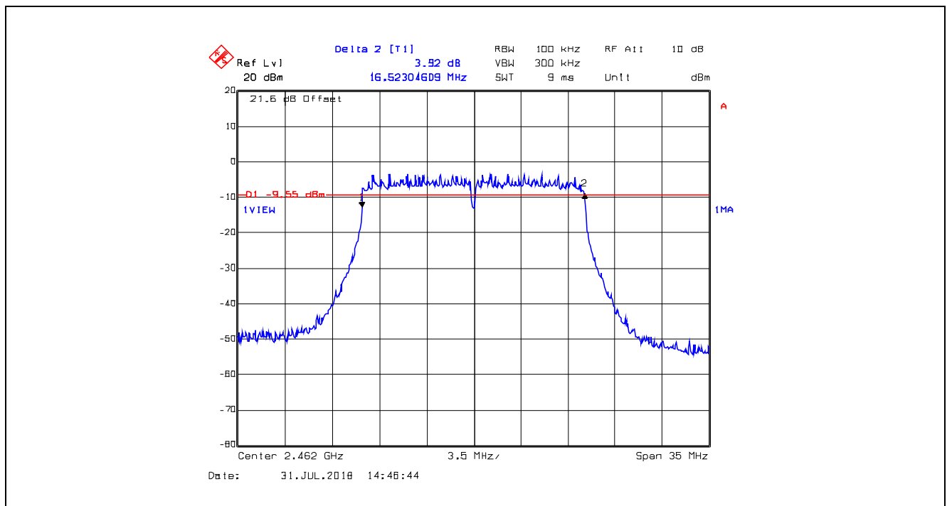
Plot 5.2.4.12. 6 dB Bandwidth, 64-QAM Modulation, 48 Mbps, Channel 11, 2462 MHz
