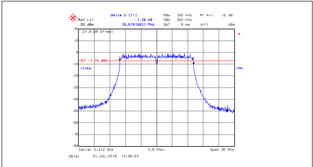
Plot 5.2.4.7. 6 dB Bandwidth, 16-QAM Modulation, 24 Mbps, Channel 1, 2412 MHz
