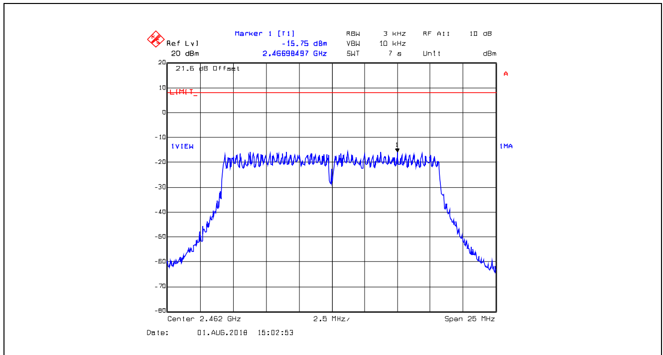
Plot 5.5.4.6. Power Spectral Density, QPSK Modulation, 12 Mbps, Channel 11, 2462 MHz
