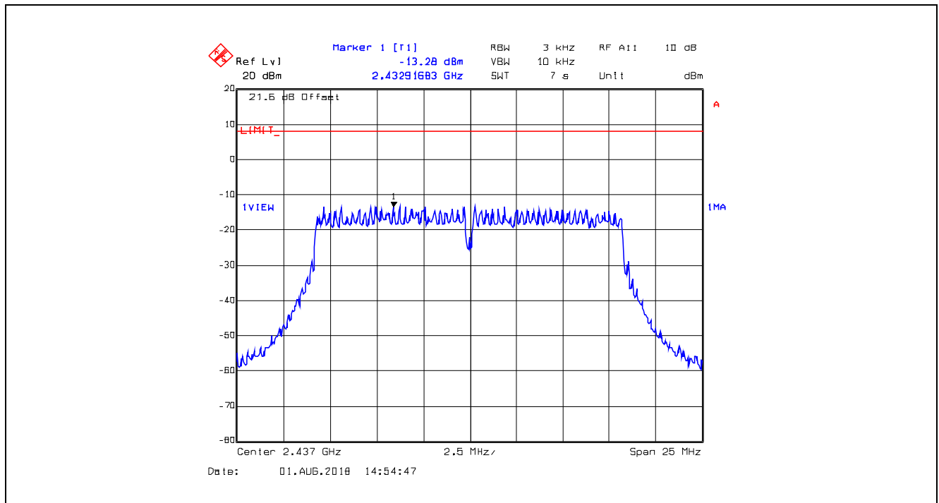
Plot 5.5.4.2. Power Spectral Density, BPSK Modulation, 6 Mbps, Channel 6, 2437 MHz
