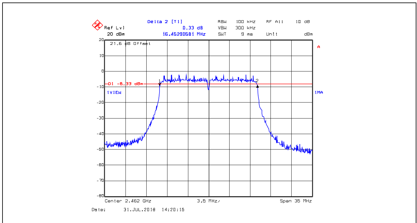
Plot 5.2.4.6. 6 dB Bandwidth, QPSK Modulation, 12 Mbps, Channel 11, 2462 MHz
