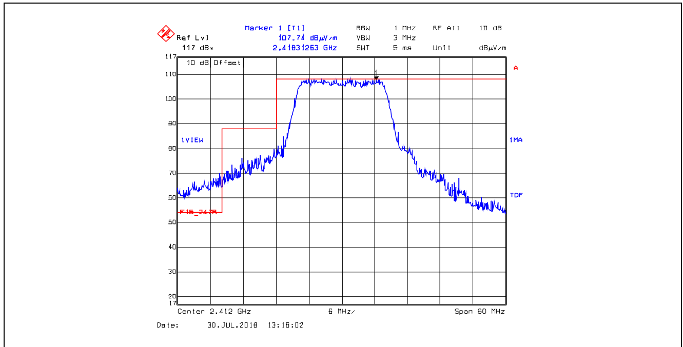
Plot 5.4.4.3.1. Band-Edge Radiated Emissions, EUT with 2.7 dBi Surface Mount Antenna, Peak Emissions Rx Antenna in Horizontal Polarization, BPSK Modulation, 6 Mbps, Ch 1, 2412 MHz
