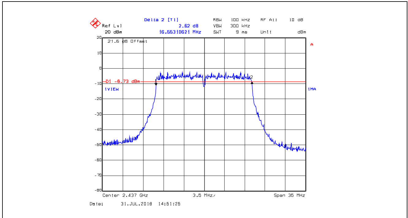
Plot 5.2.4.11. 6 dB Bandwidth, 64-QAM Modulation, 48 Mbps, Channel 6, 2437 MHz
