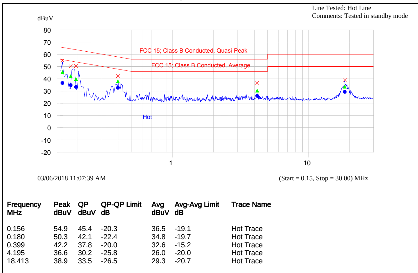
Plot 5.1.3.1. Power Line Conducted Emissions –Standby Mode
