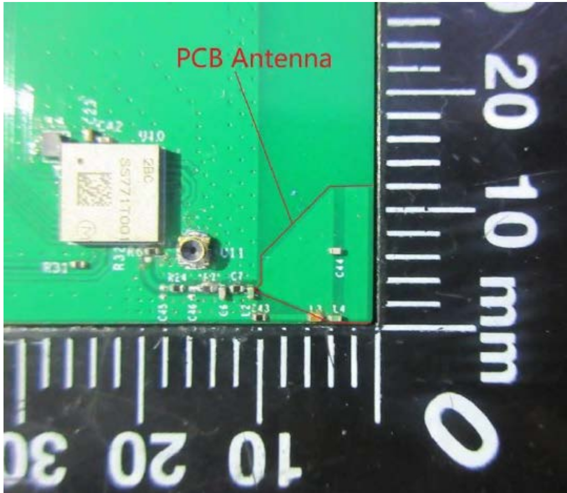
PCB Antenna
