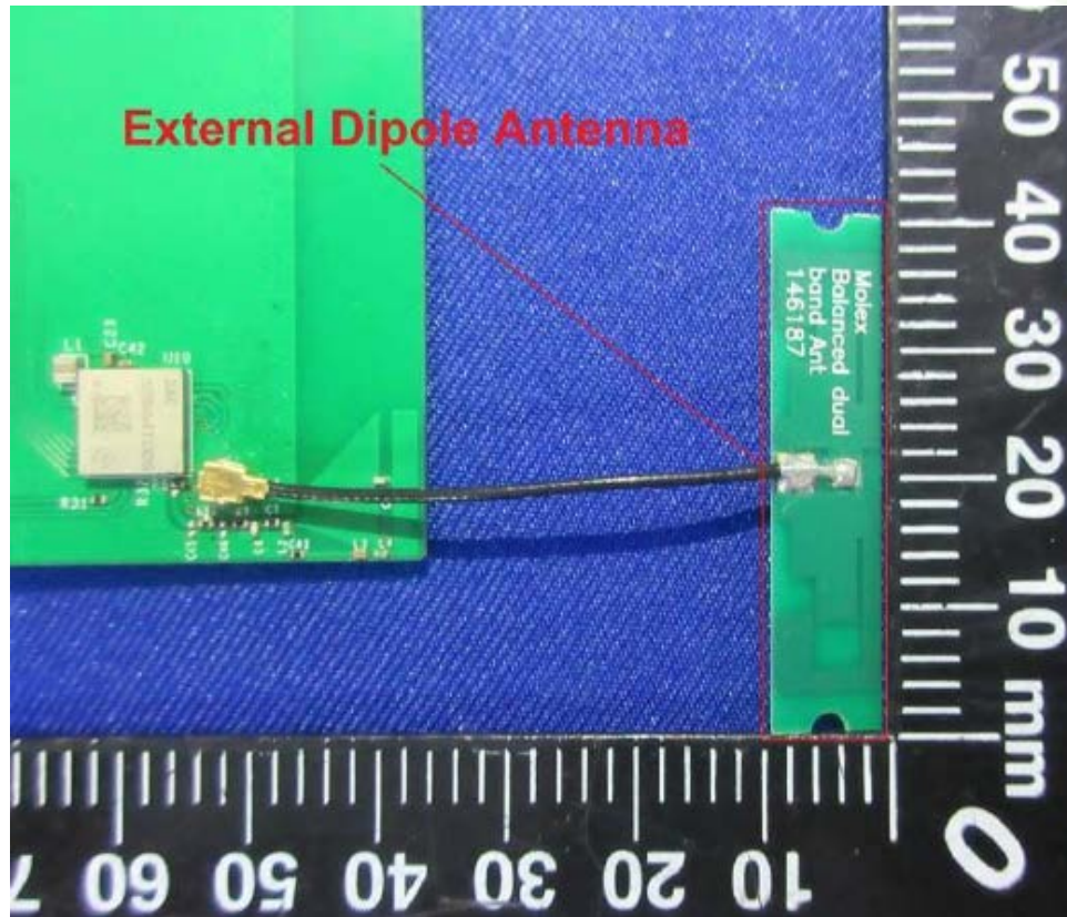
External Dipole Antenna-1
