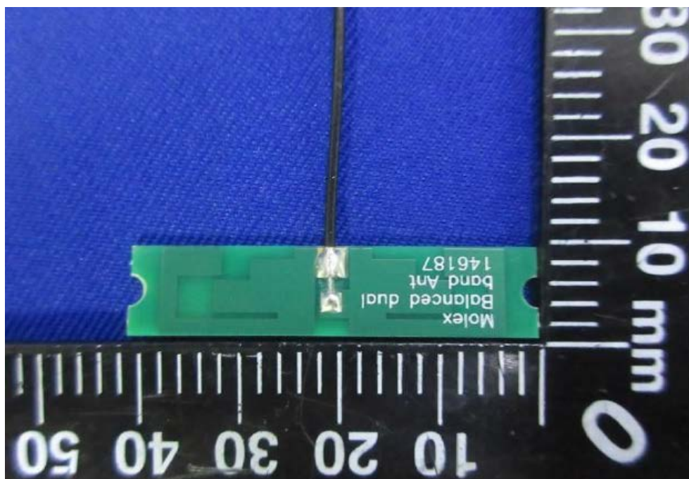
External Dipole Antenna-2
