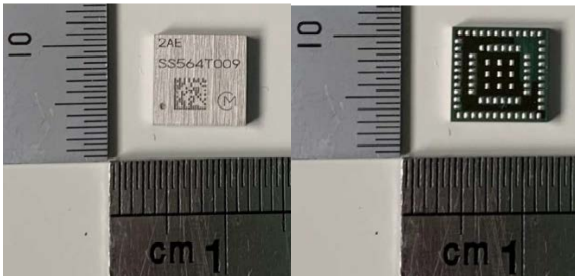
Radio Module (Top and Bottom views)
