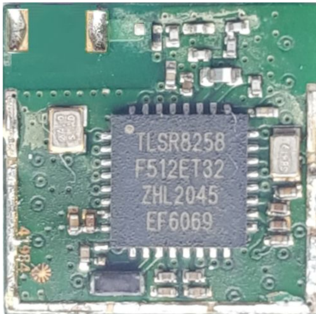
Module Front w/o shielding
