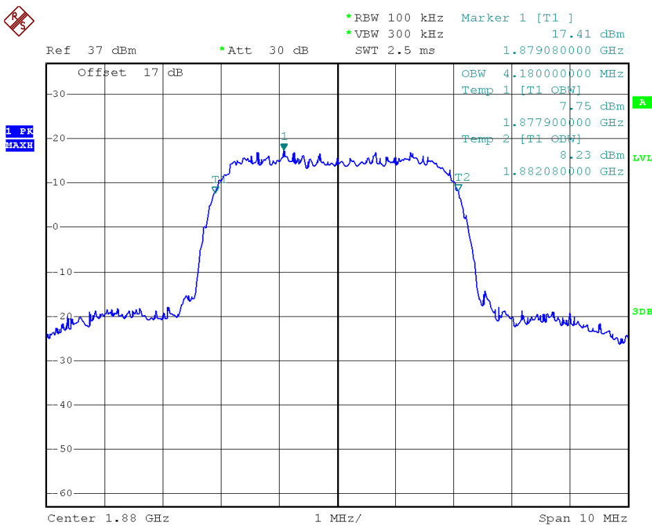
(Plot F4: WCDMA 1900MHz Channel = 9400 99% Occupied Bandwidth)
