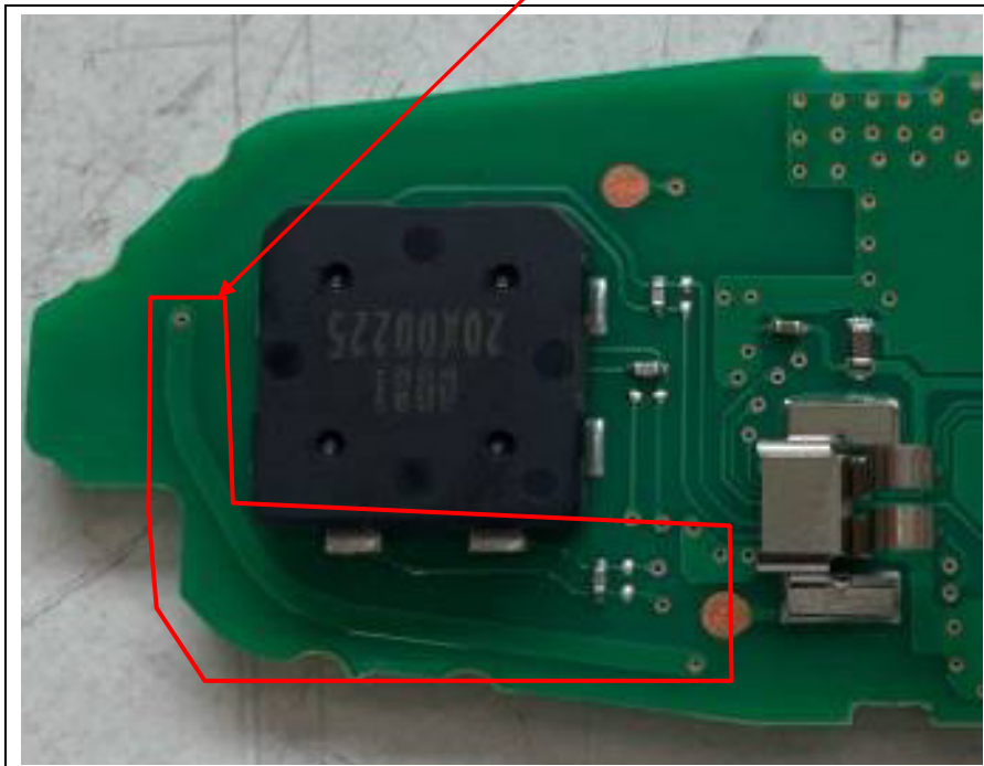
PCB Pattern Antenna
