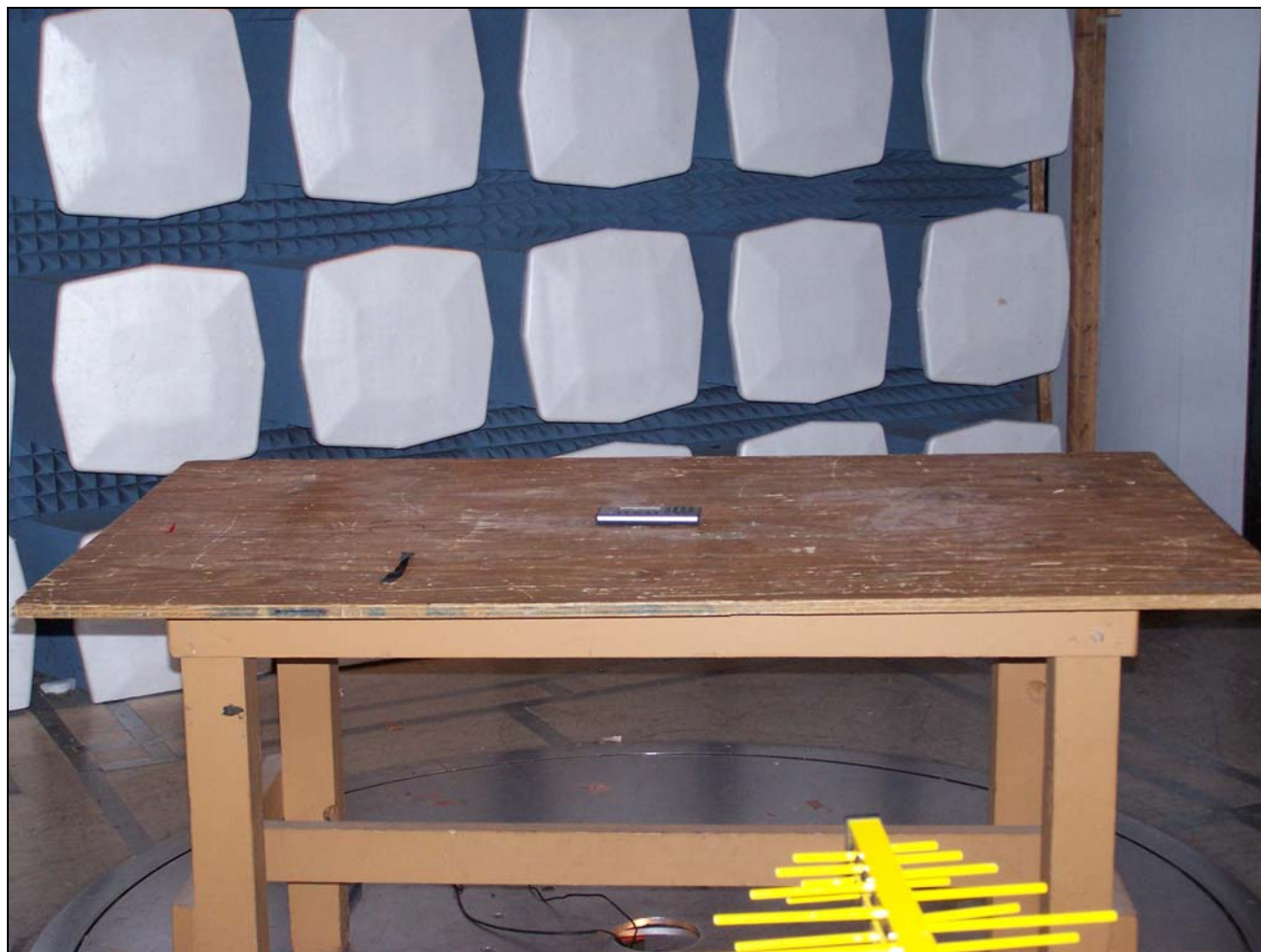
Photograph 1. View, Radiated Emission Limits, Test Setup
