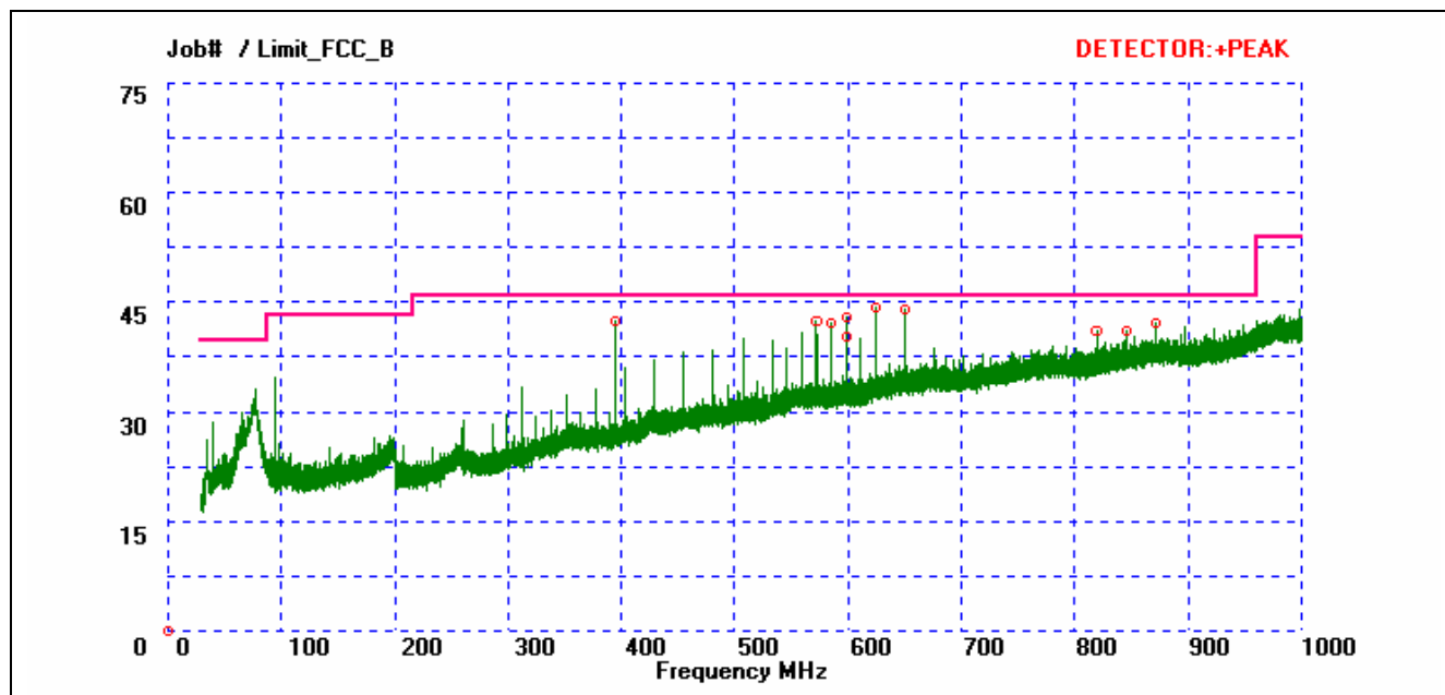
Plot 1. Radiated Emission Limits, Test Setup
