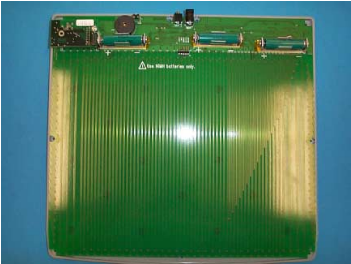
Bottom of PCB with Bluetooth module
