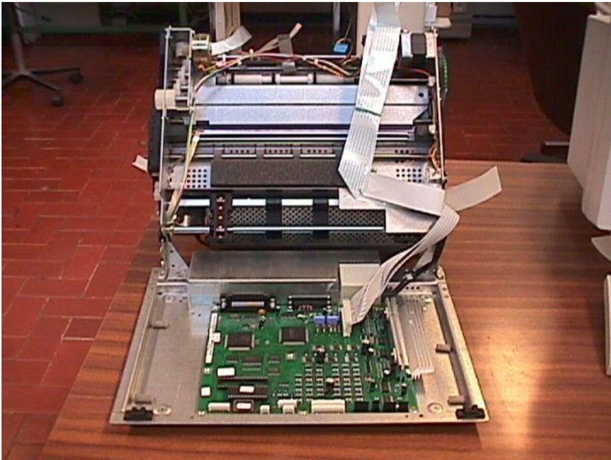
picture 4: electronic board in its stand
