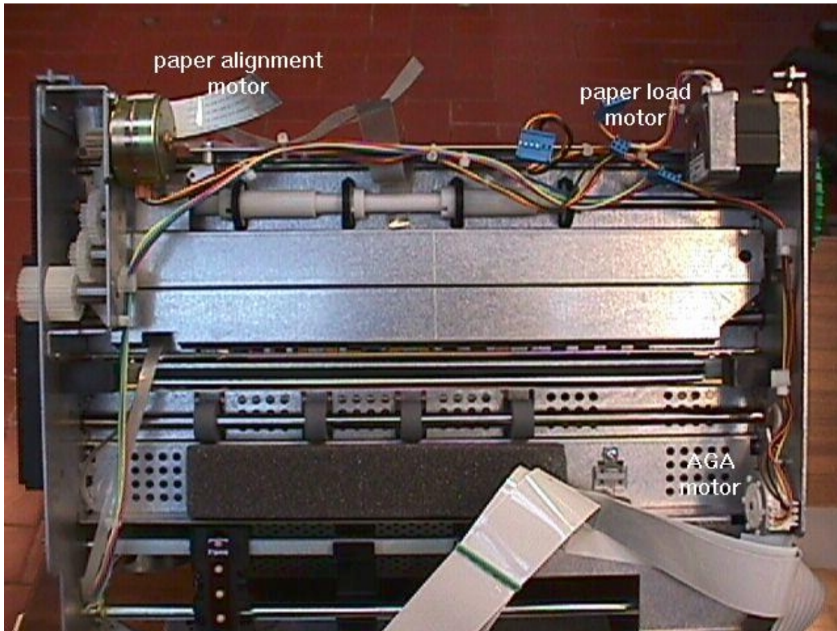
picture 5: step motors
