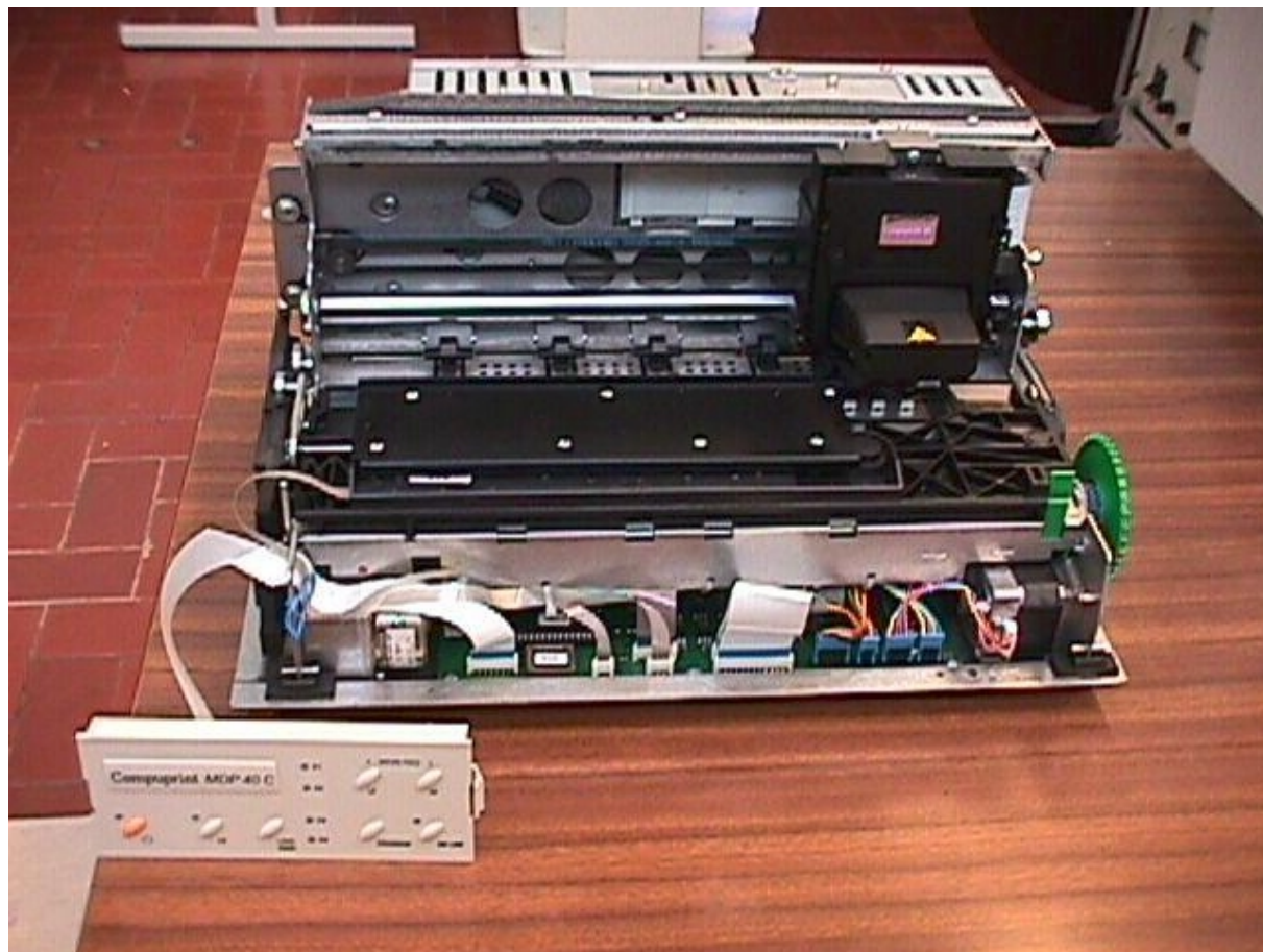
picture 1: front view without shell
