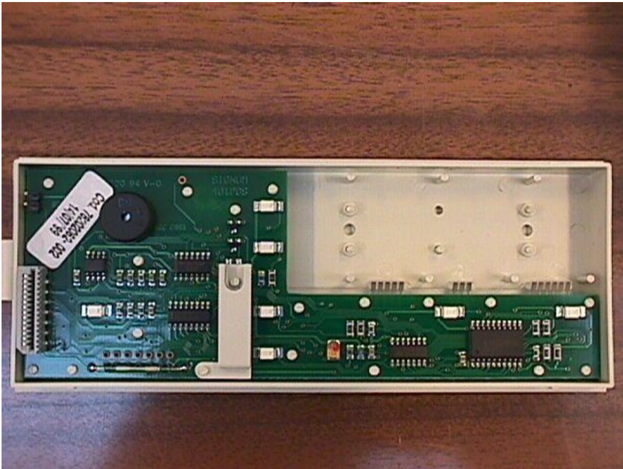
picture 14: Operator panel board
