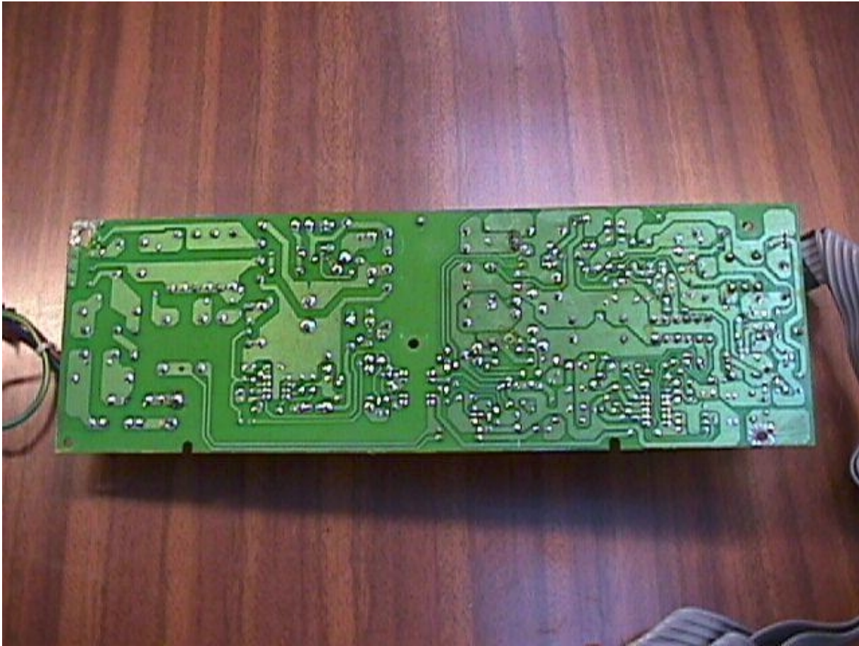
picture 12: power supply board solder side
