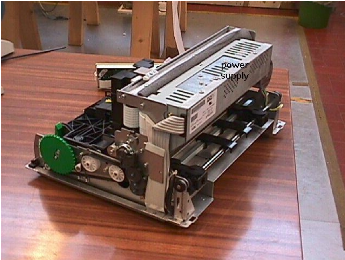
picture 2: rear view without shell
