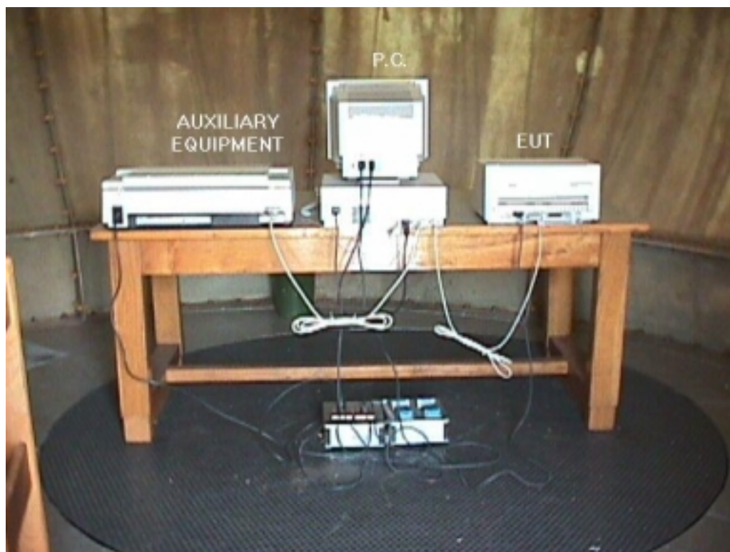
picture 6: radiated measurements rear view parallel (CENTRONICS) transmission
