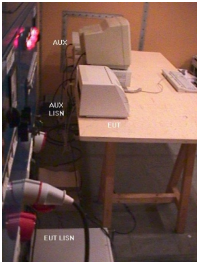
picture 2: conducted measurement rear view serial transmission
