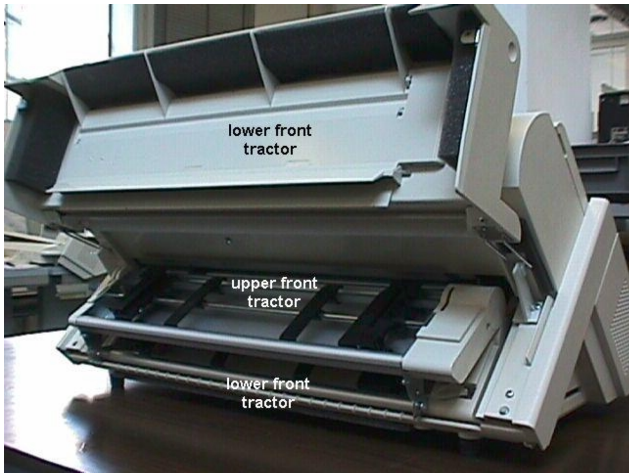
picture 5: front view with the front tractors cover open
