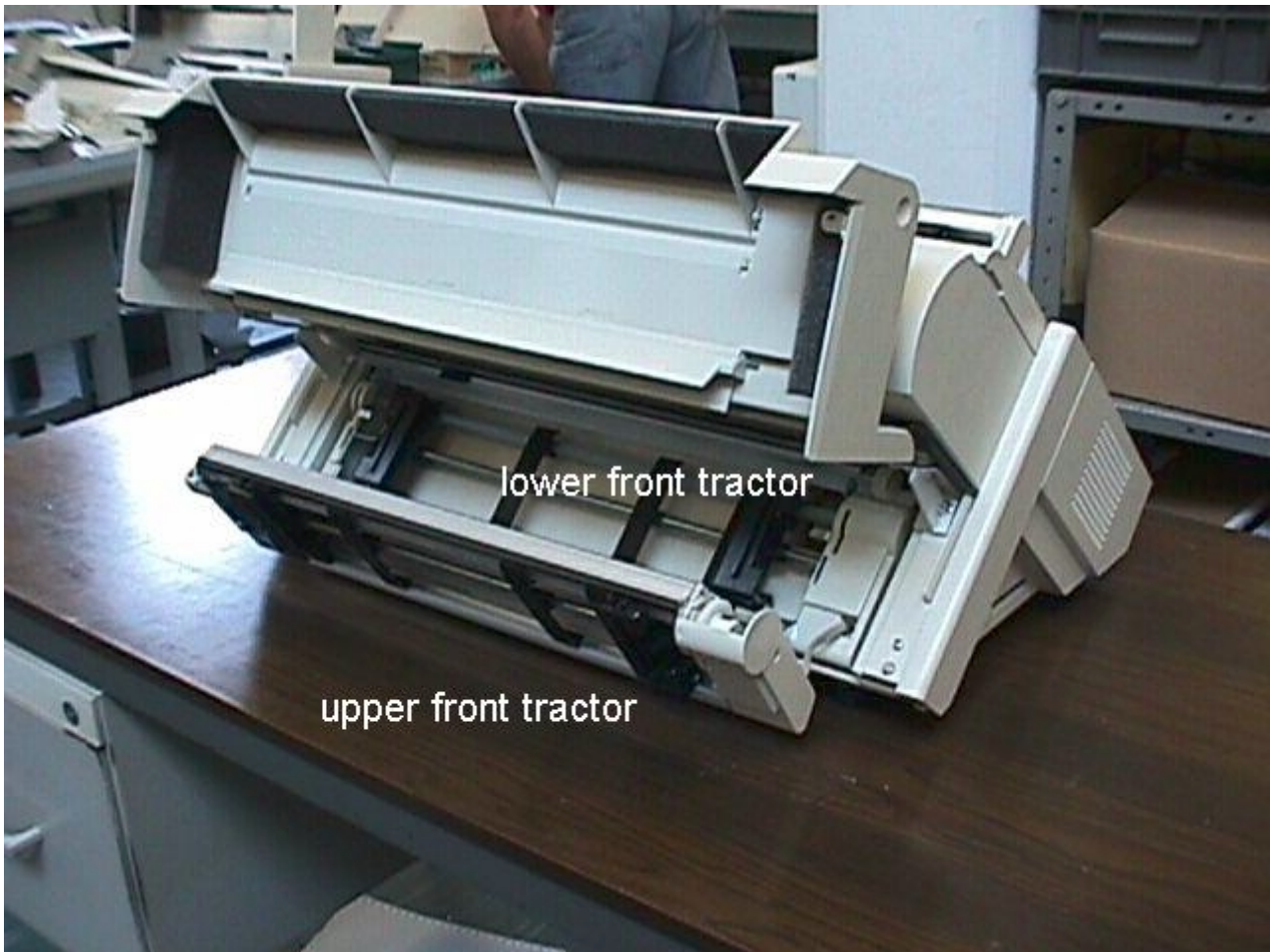
picture 6: front view with the upper front tractor released
