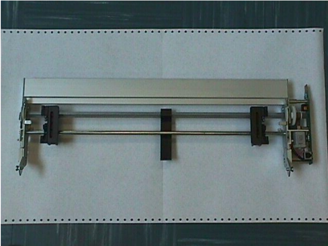
picture 15: front lower tractor assy: the board is right side
