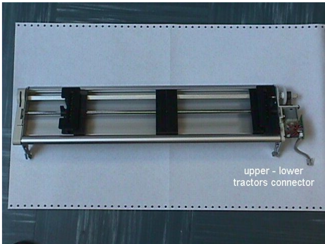
picture 16: front upper tractor assy
