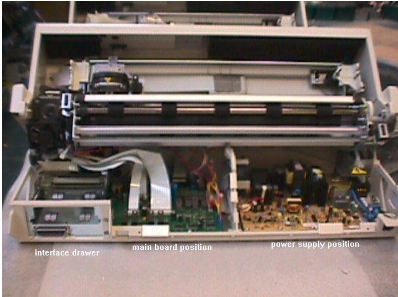
picture 1: electronic boards in their stand
