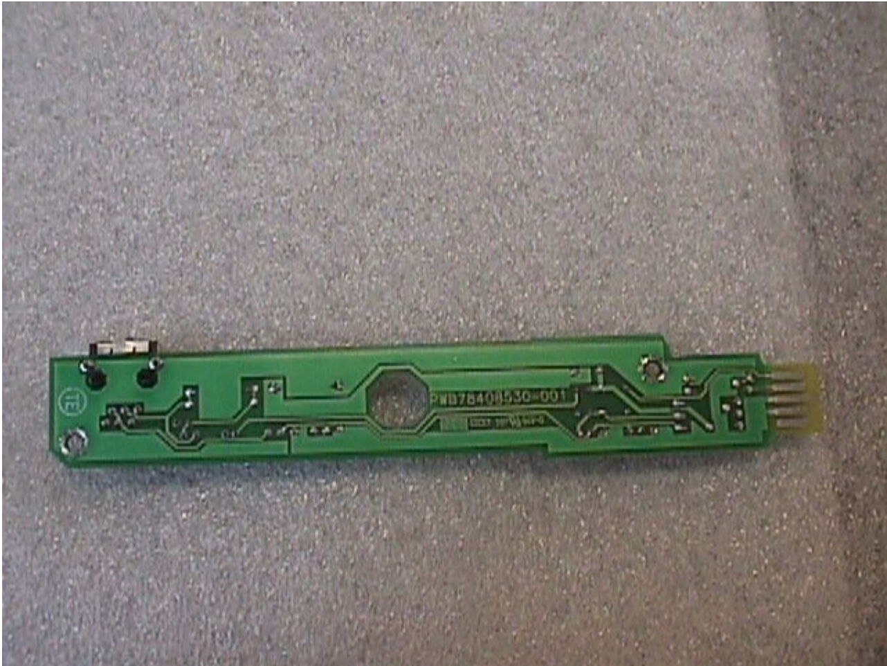
picture 14: front lower tractor board solder side
