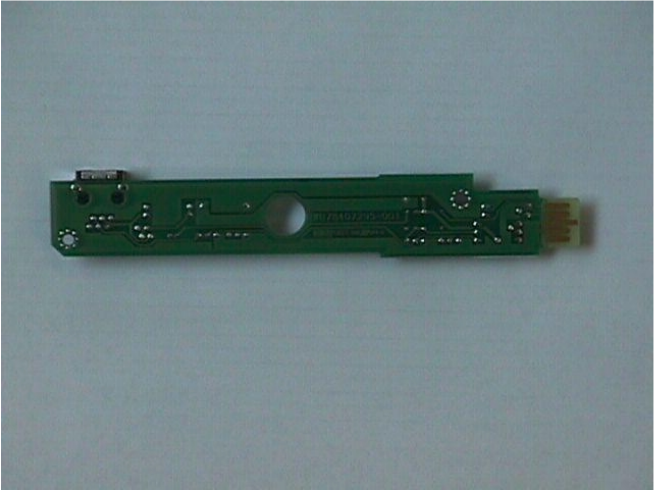
picture 12: front lower tractor board solder side
