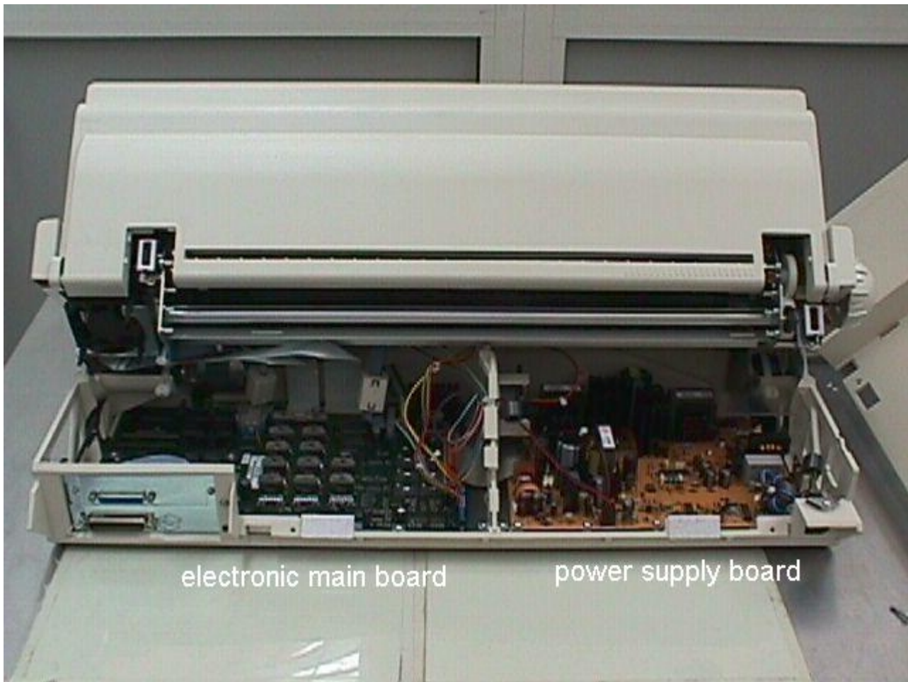
picture 1: electronic assembly: boards in their stand
