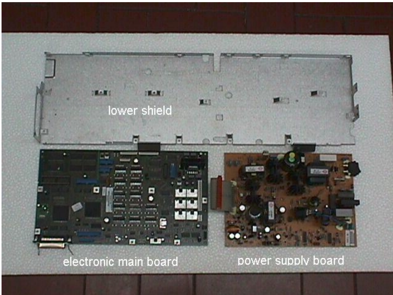
picture 2: electronic boards and shield out of the mechanical assy
