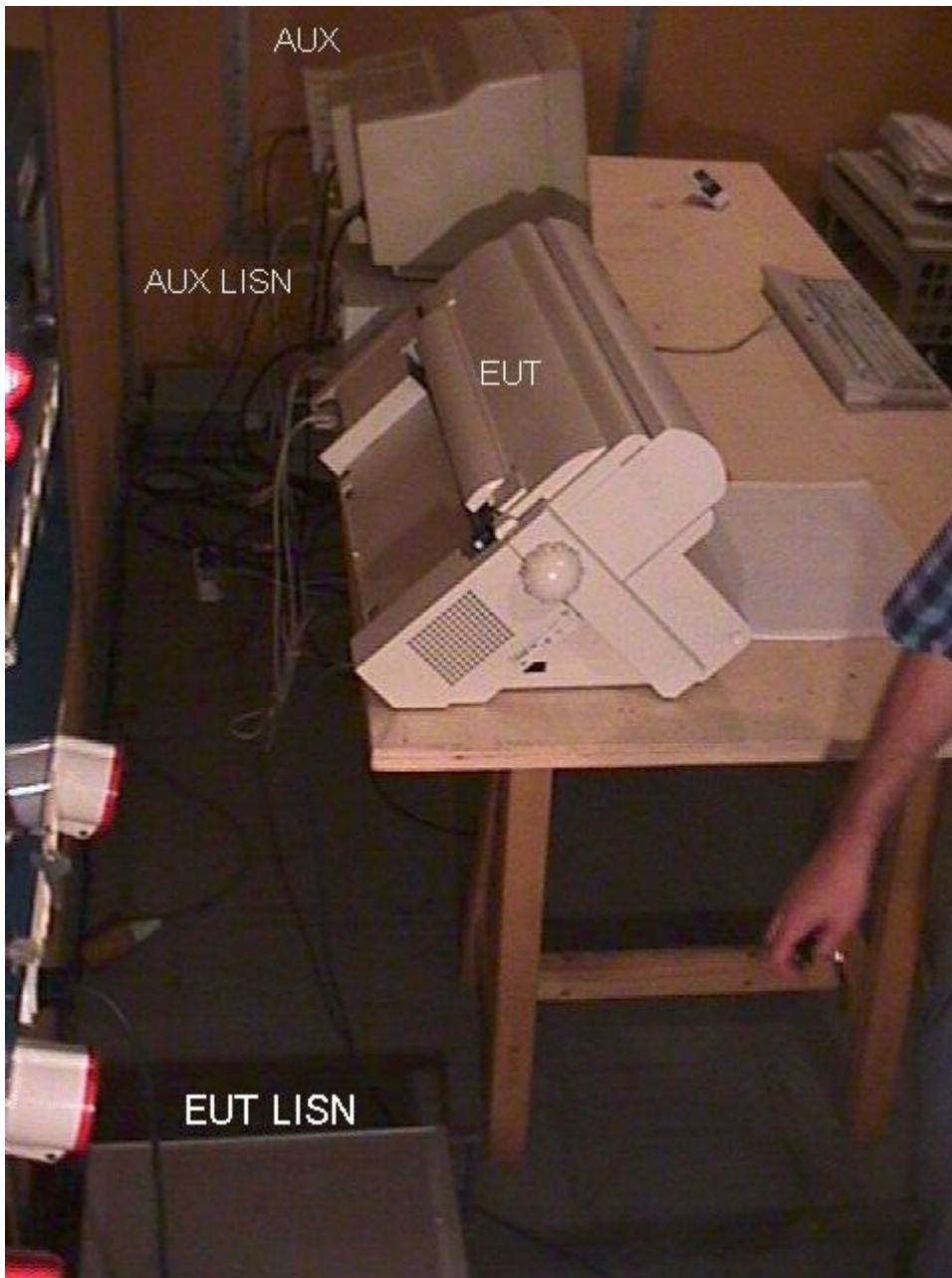
picture 2: conducted measurement rear view serial transmission
