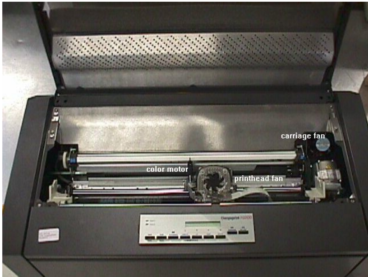
picture 6 : upper view with the upper cover open
