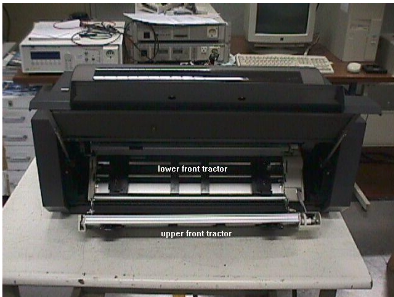
picture 5 : front view with the upper front tractor released
