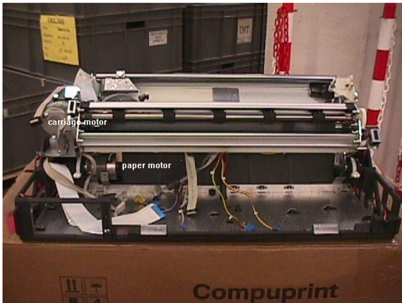
picture 2 : lower shield without boards and interface drawer
