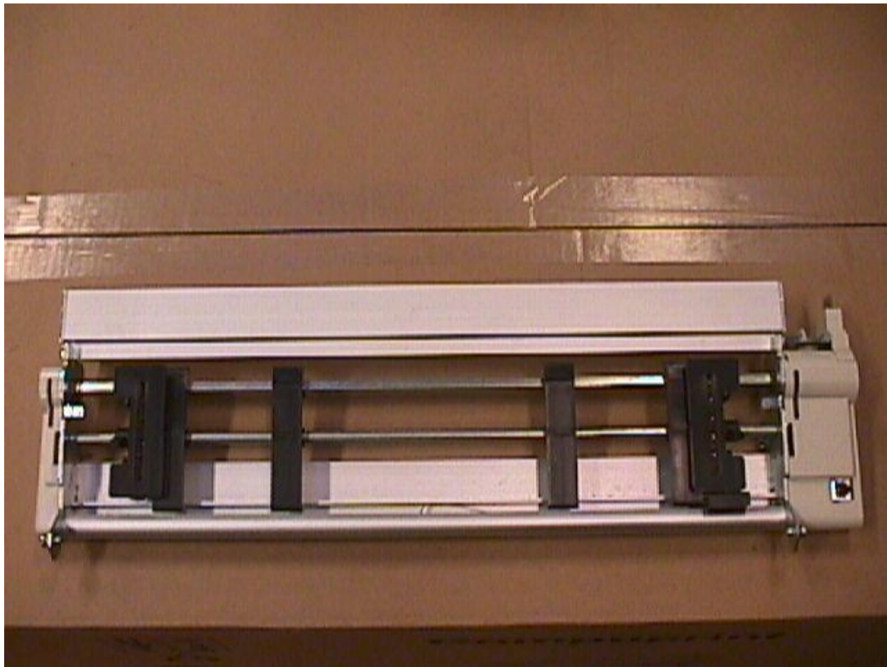
picture 17 : front lower tractor assy
