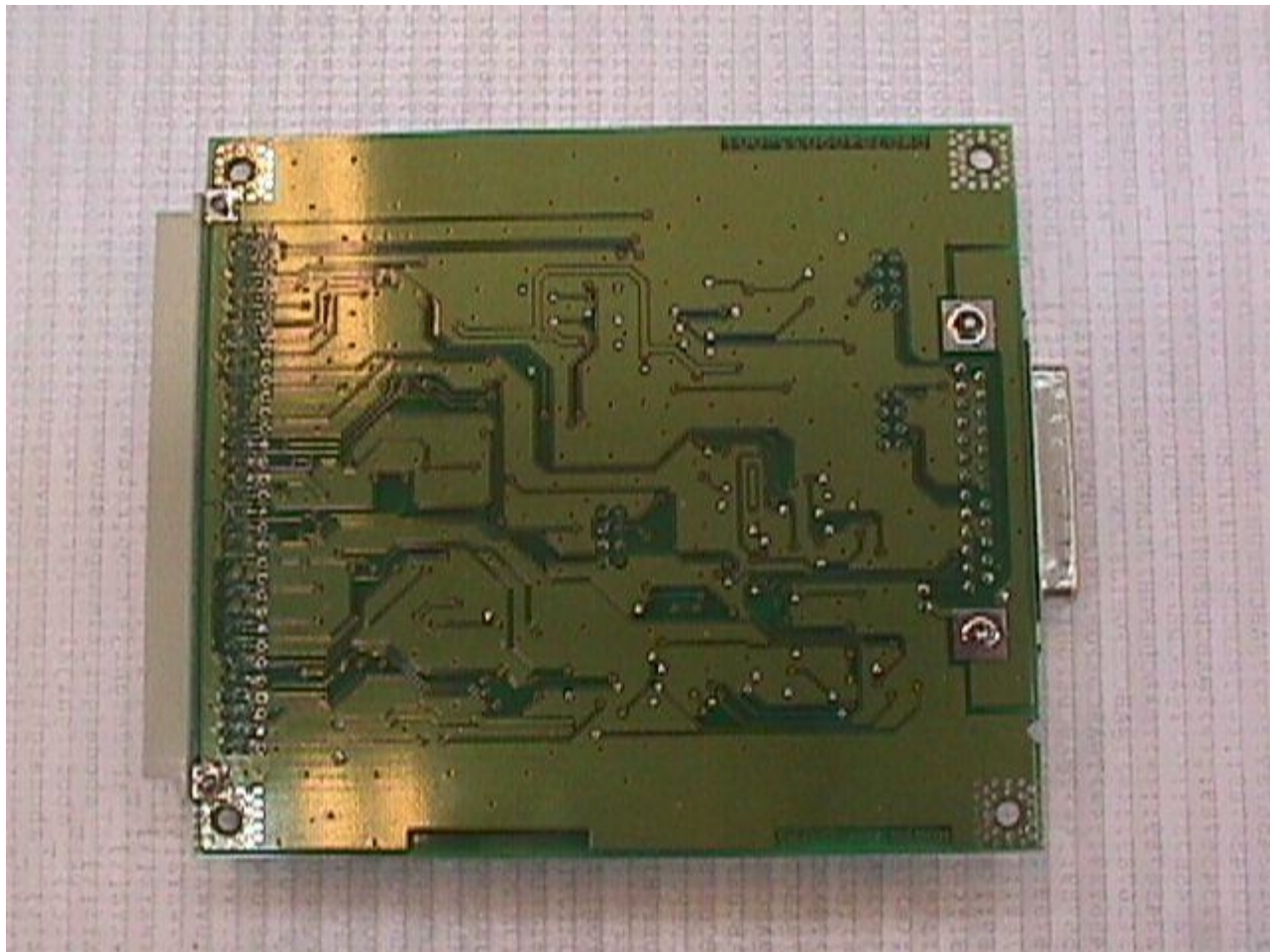
picture 13 : optional serial interface solder side
