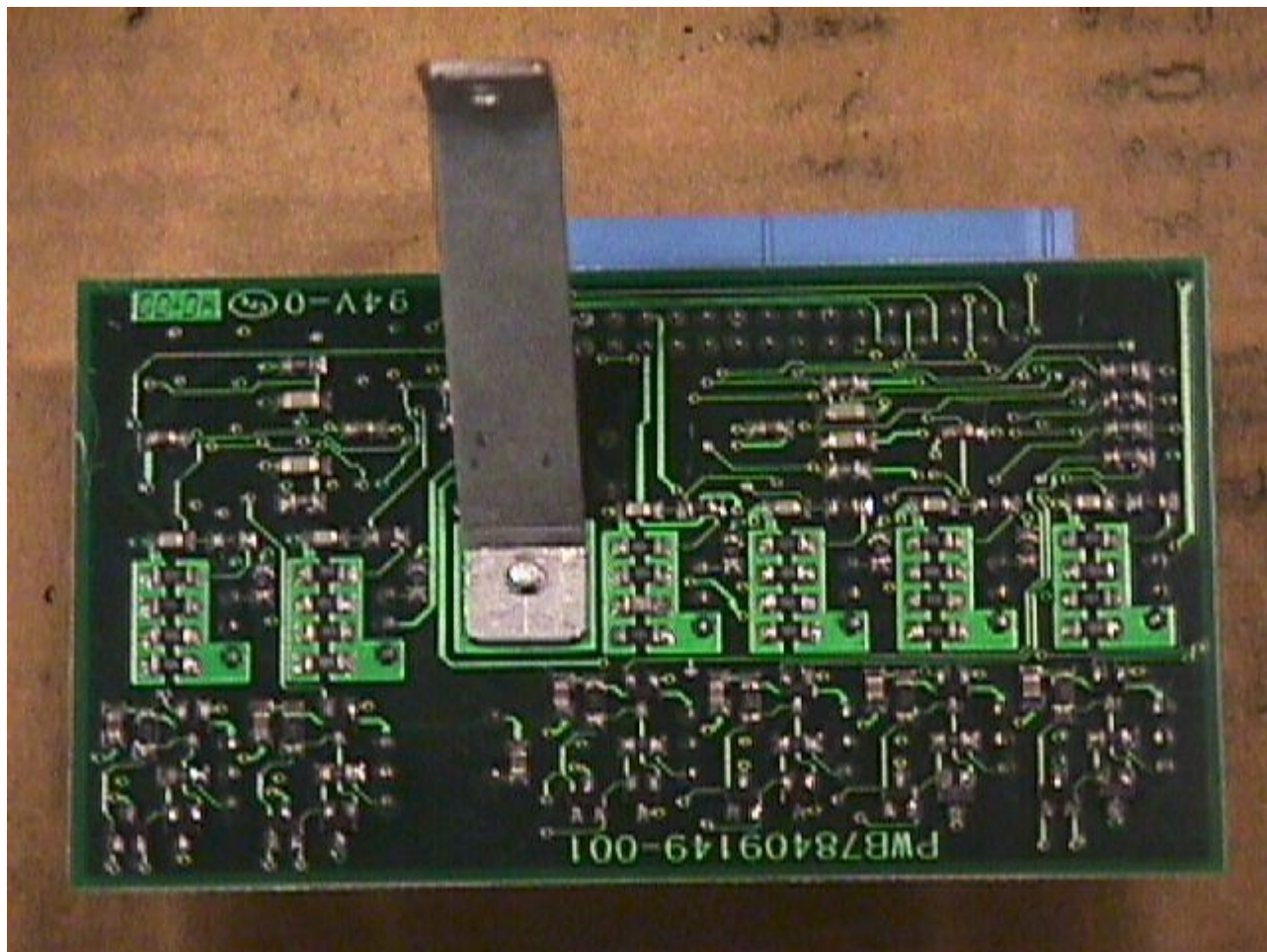
picture 11 : additional needle board solder side
