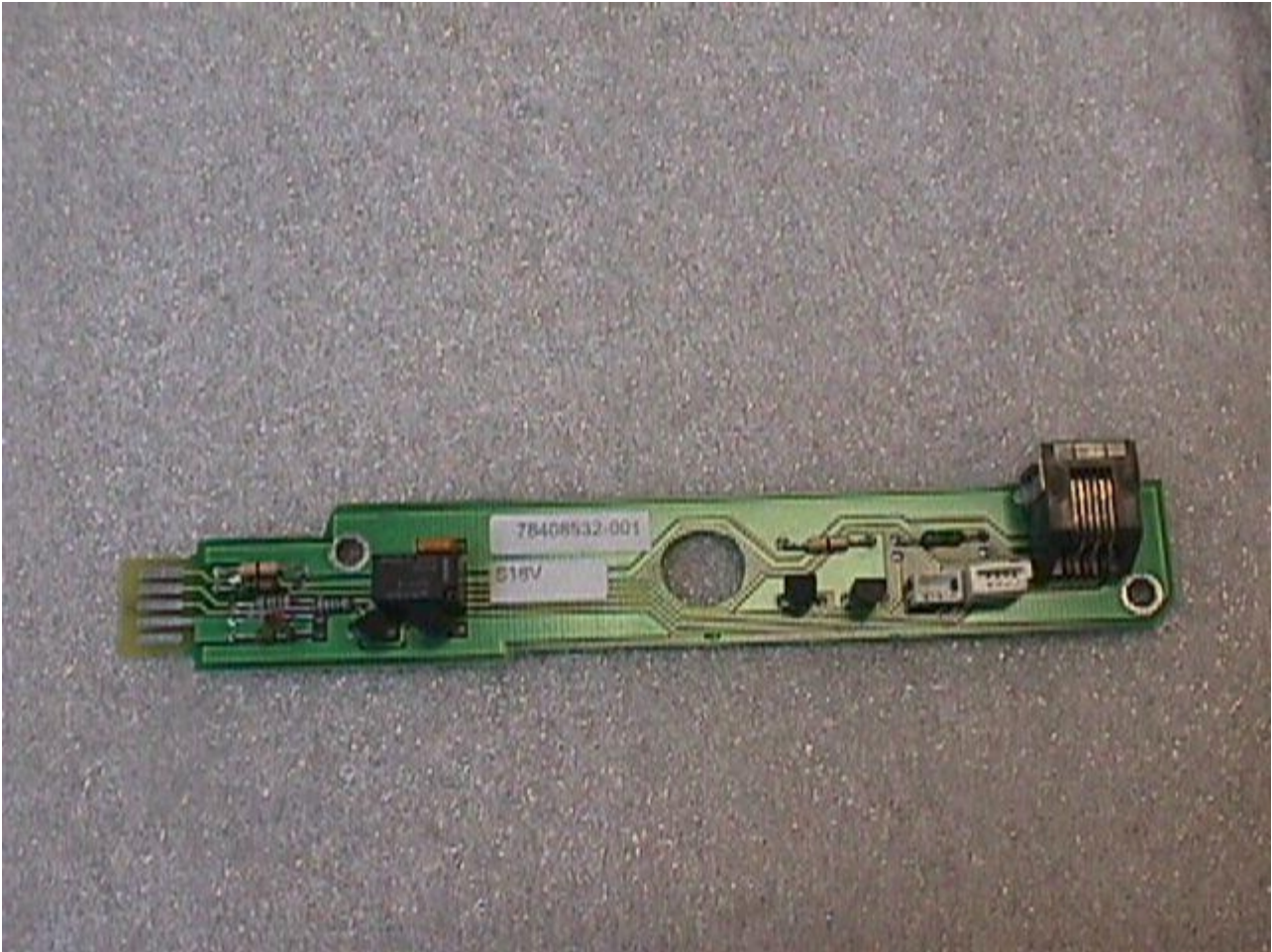
picture 15 : front lower tractor board component side
