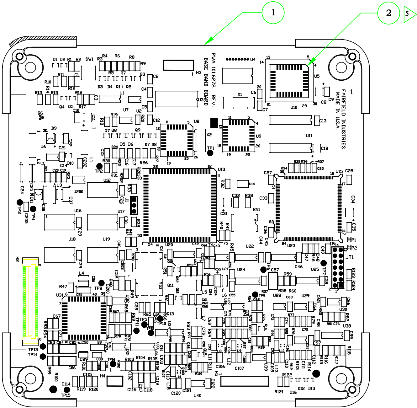
PRIMARY SIDE
