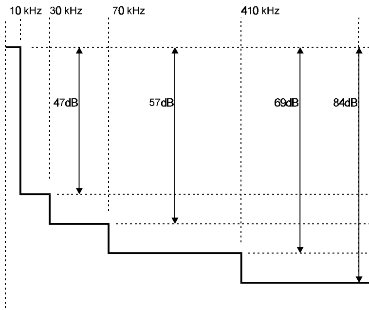
Transmitter Mask
