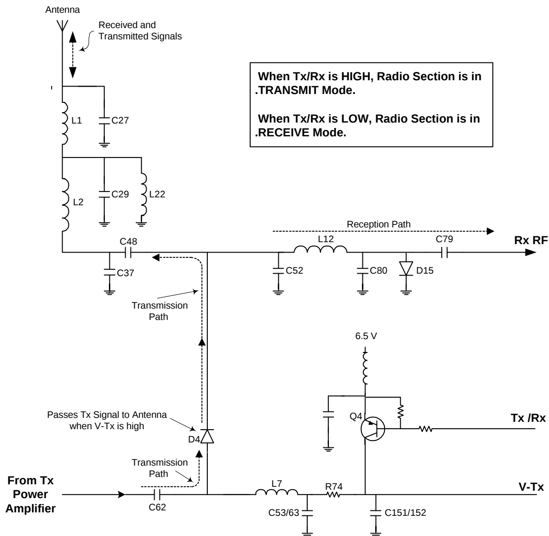
Transmit/Receive Switch & RF Paths to and from Antenna Figure 6
