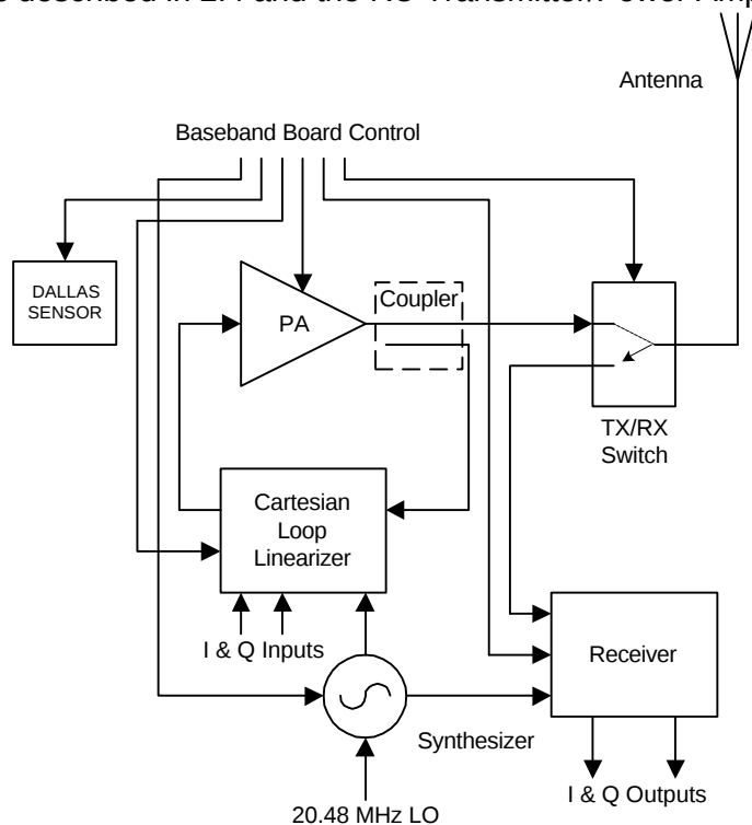
Remote Unit RF Module Overall Block Diagram
