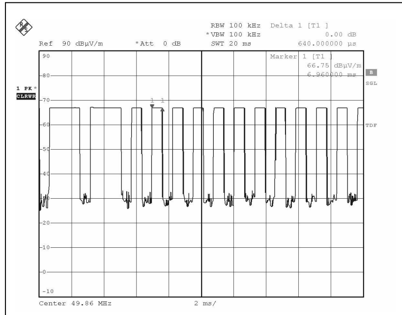
Duty Cycle 3
