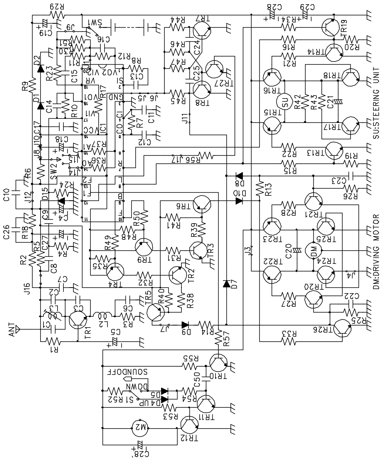
NO.RP6430 CIRCUIT DIAGRAM (FCC ID:CVTRP6430H)
