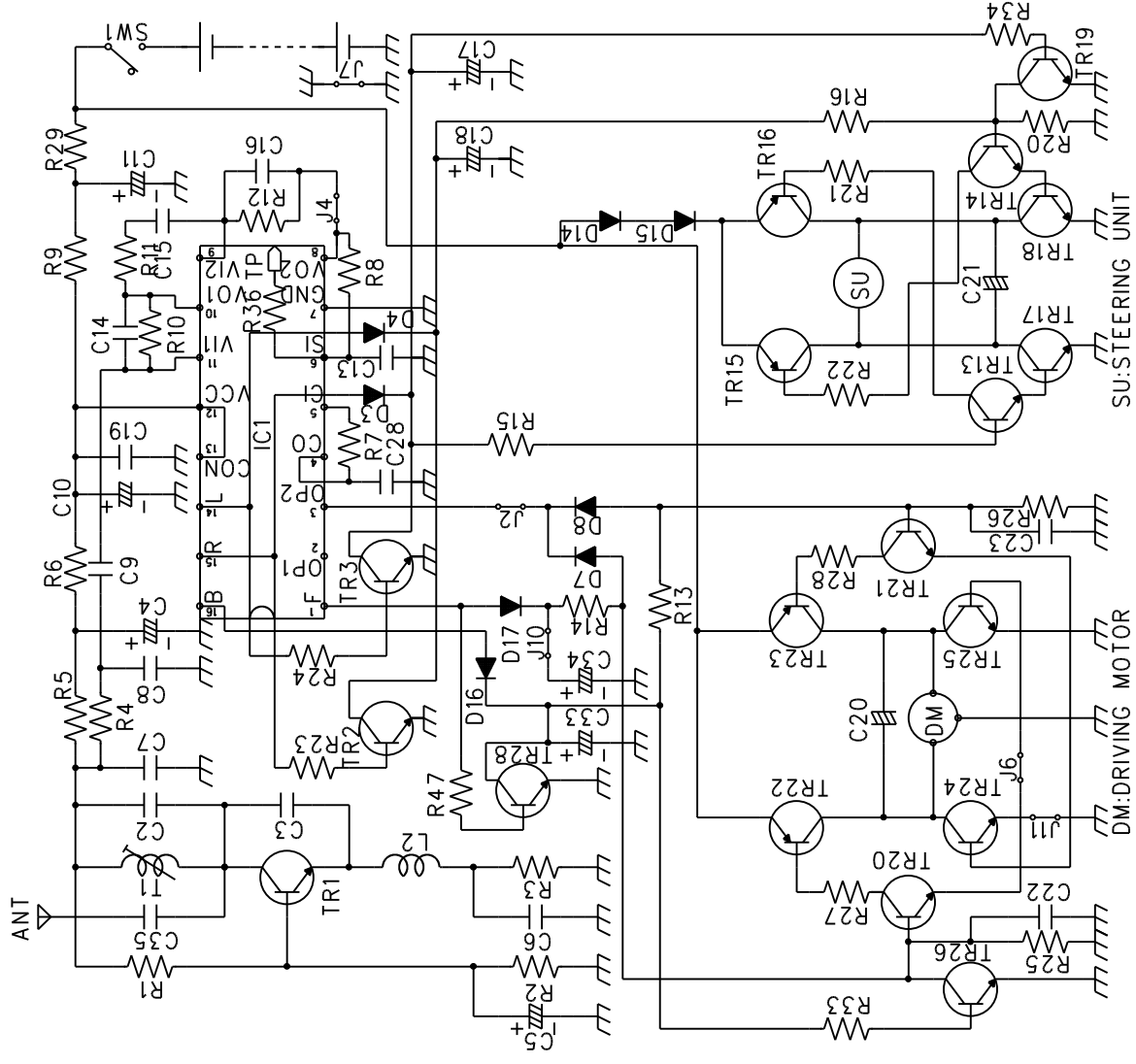
NO.RP6440 CIRCUIT DIAGRAM
