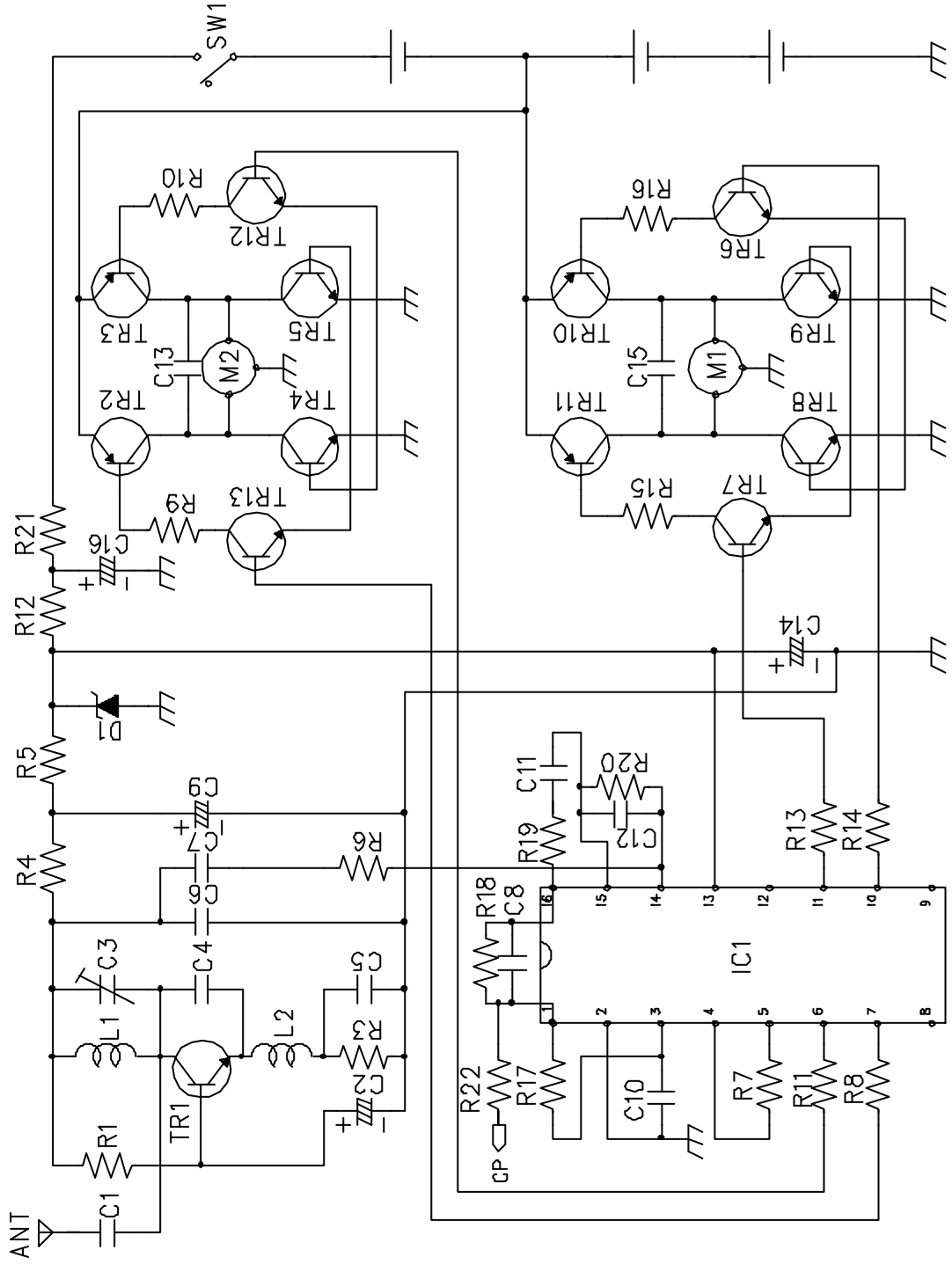
NO.RP7430 CIRCUIT DIAGRAM
