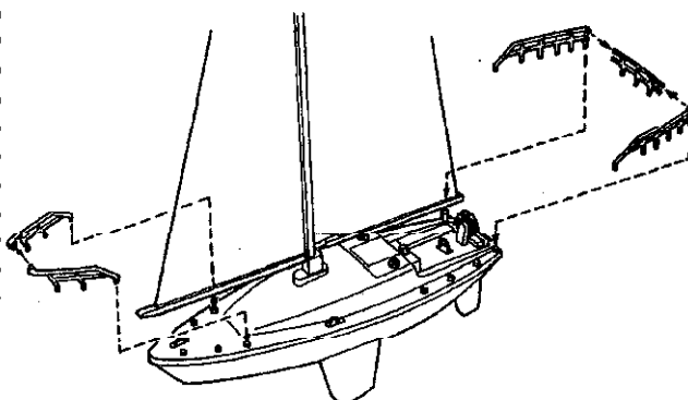
Mount hand-rails.
