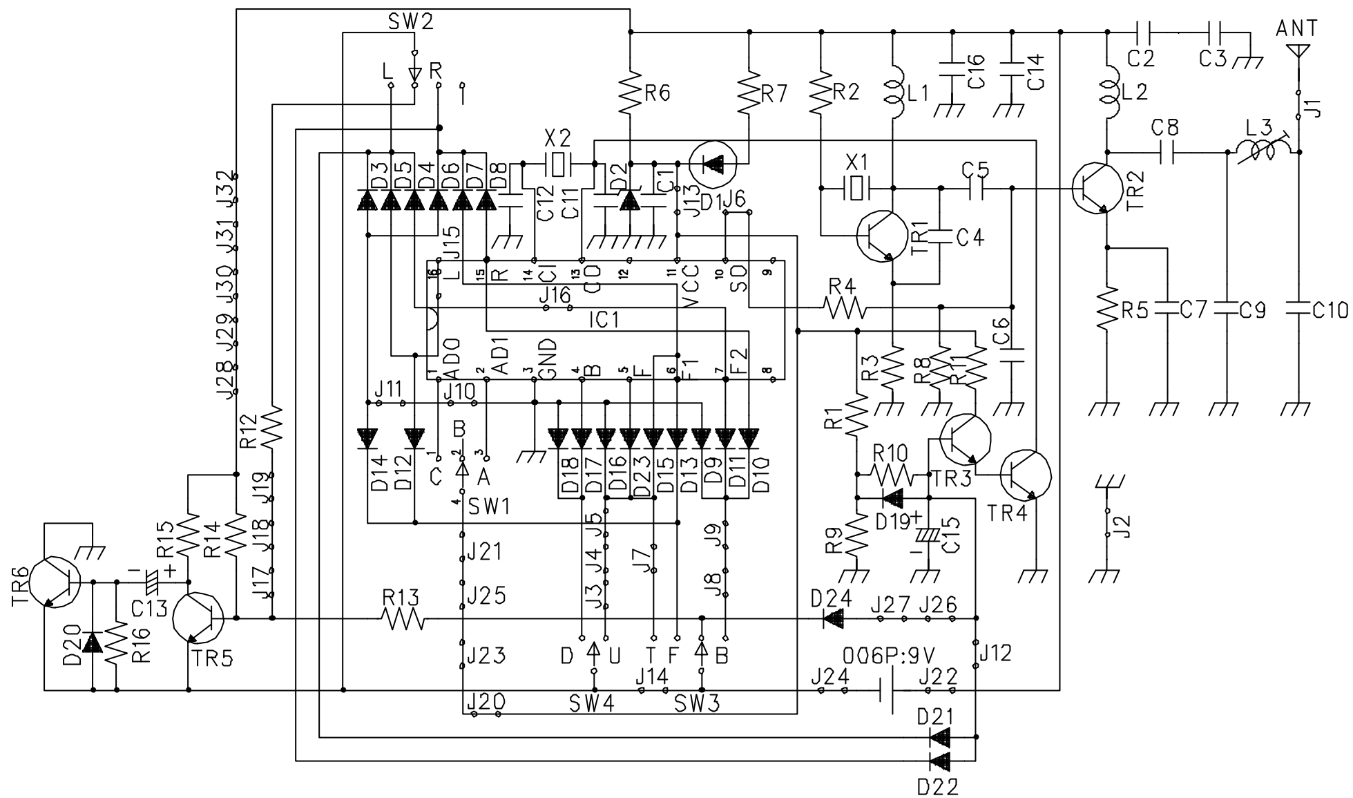
NO.TP6793 CIRCUIT DIAGRAM
