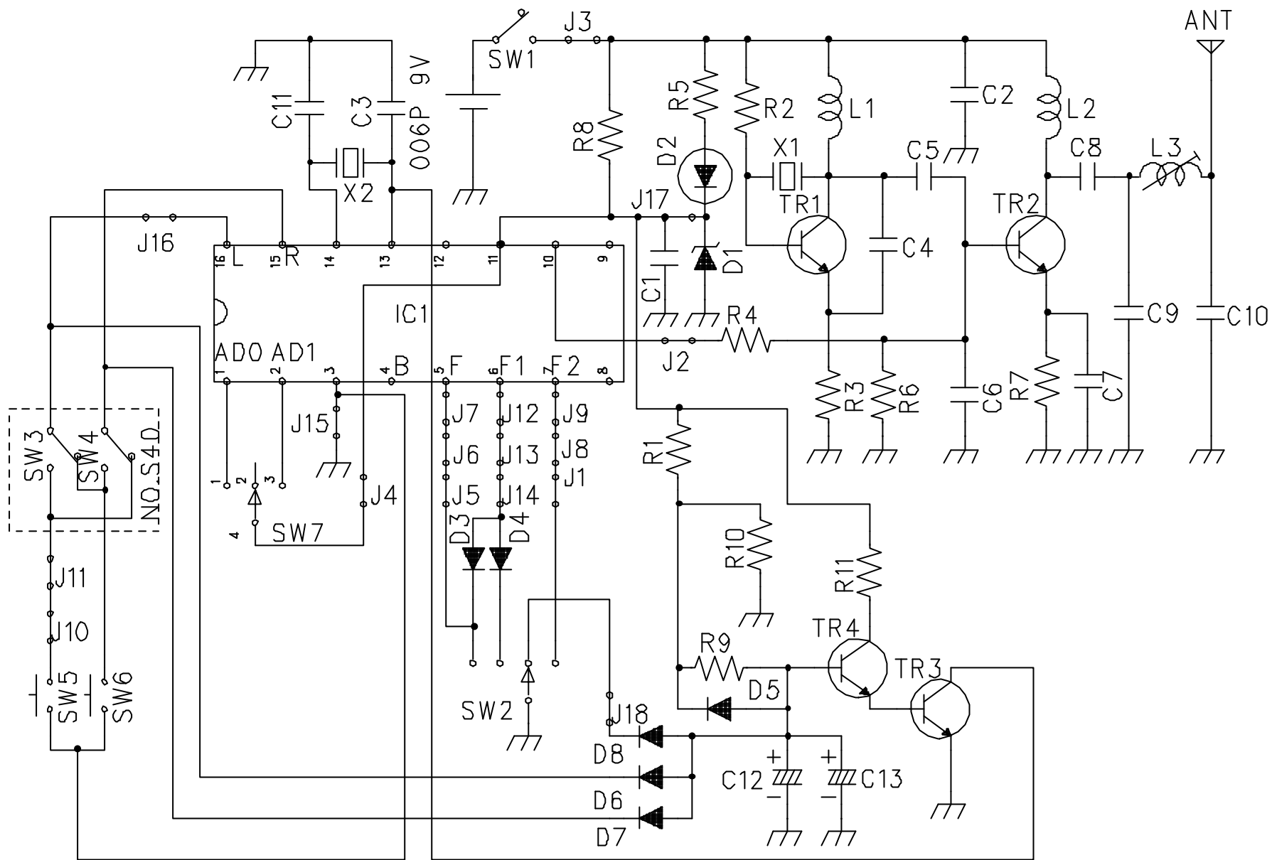
NO.TP8501 CIRCUIT DIAGRAM (FCC ID:CVTTP8501)
