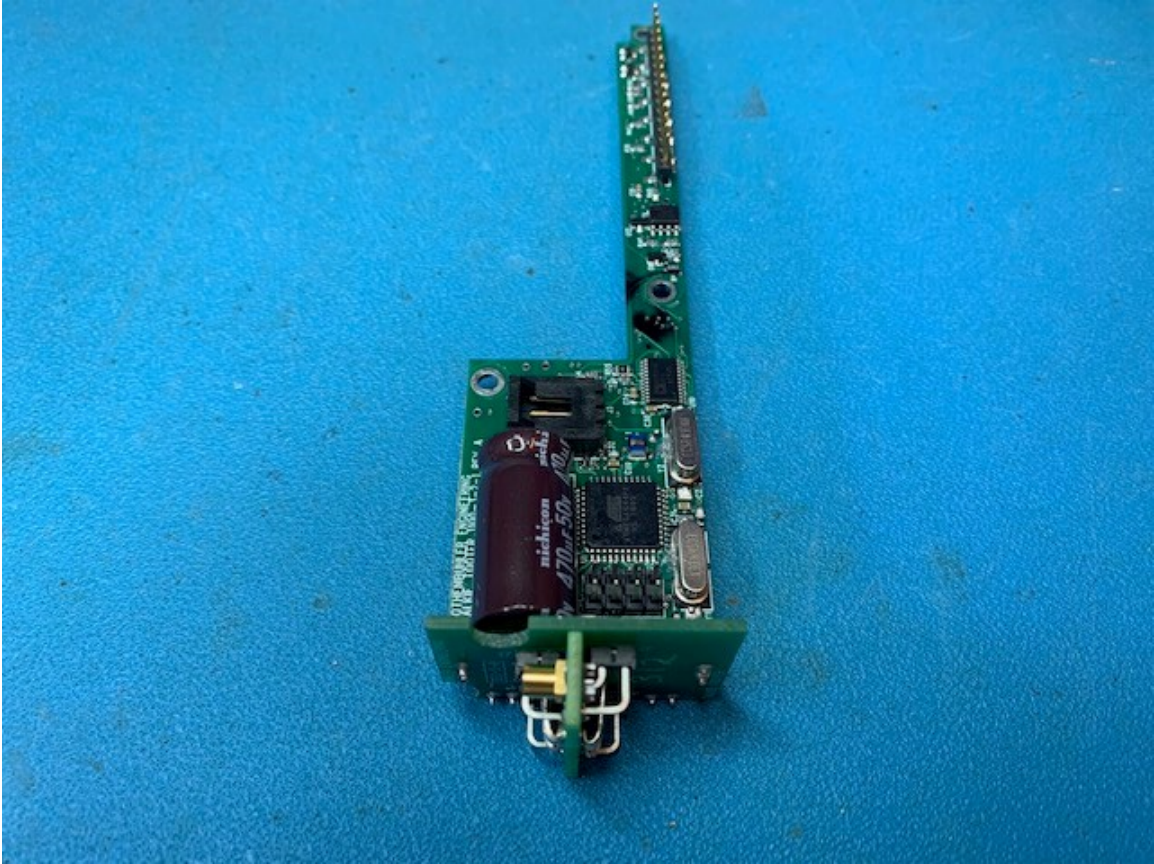
Picture 3 1100-3-2 Antenna Interface End View
