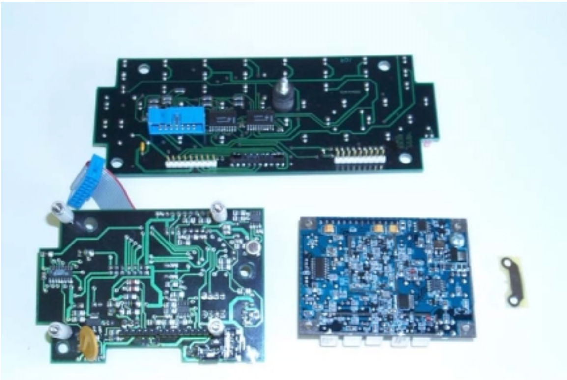
Figure 2. Bottom Side Of 1668-1 Circuit Board Assemblies
