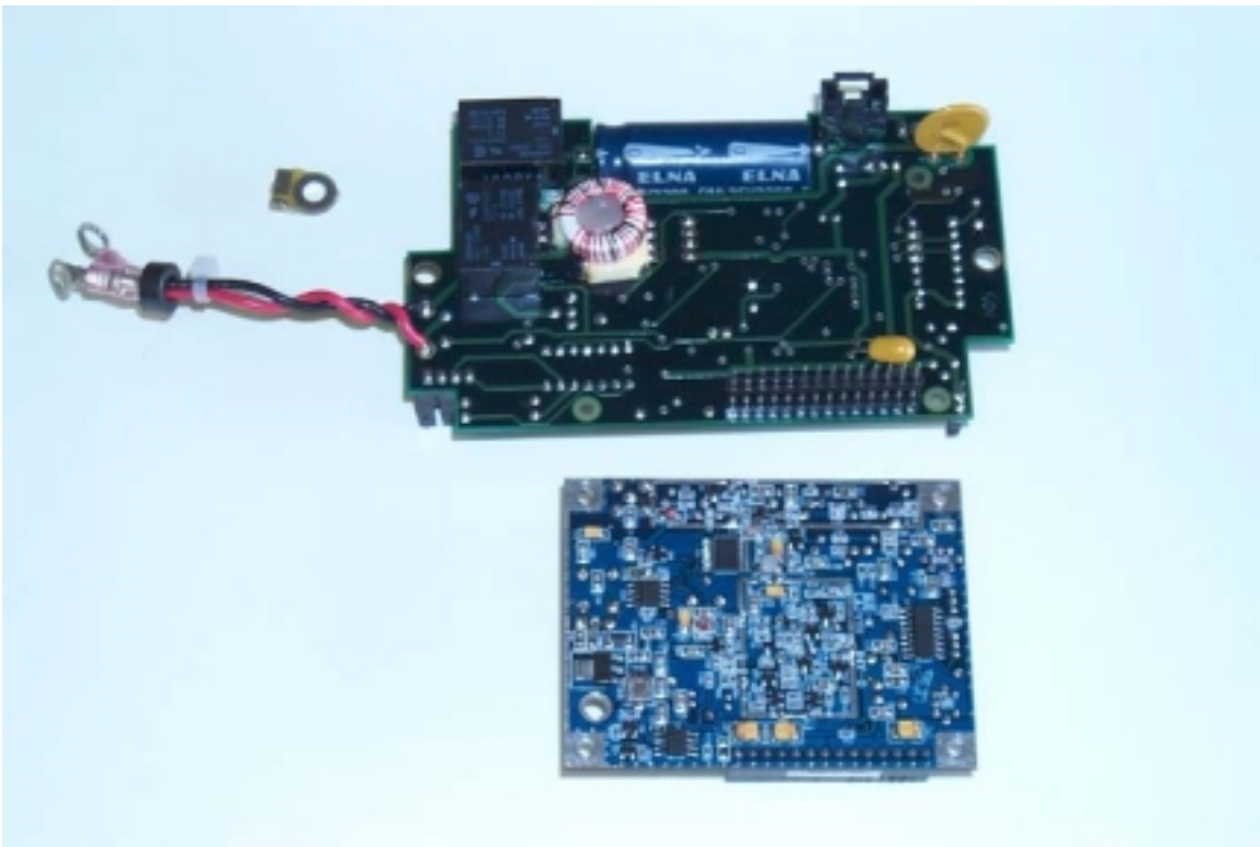
Figure 2. Bottom Side of 1668-2 Circuit Boards
