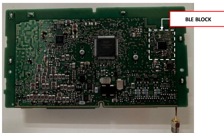
Bottom View without cover
