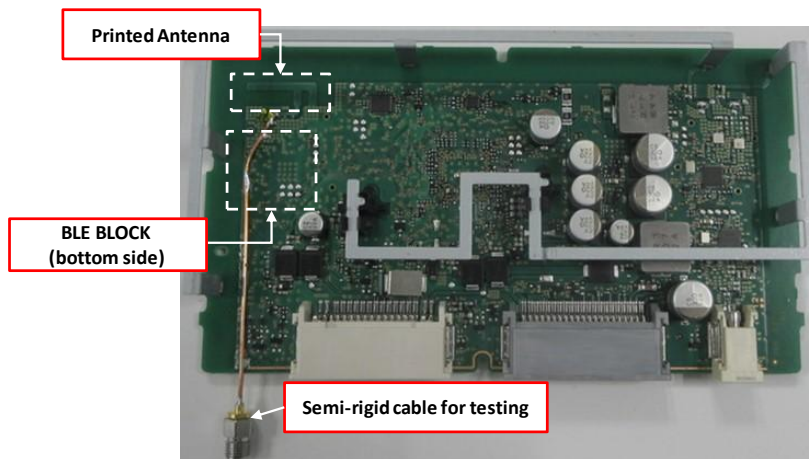
TOP View without cover
