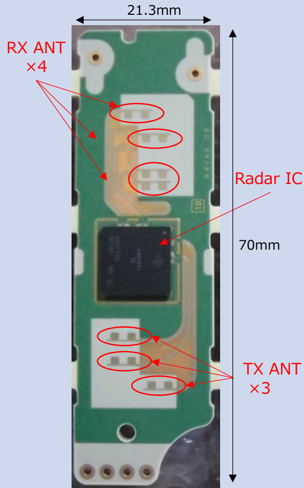
Reverse Side w/o Shield
