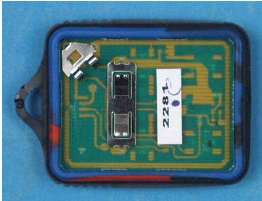
Interior circuit, back
