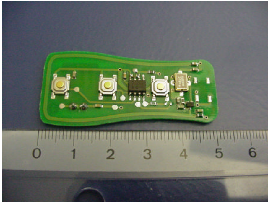
Picture 3 : vehicle remote keyless entry transmitter, view to the PCB
